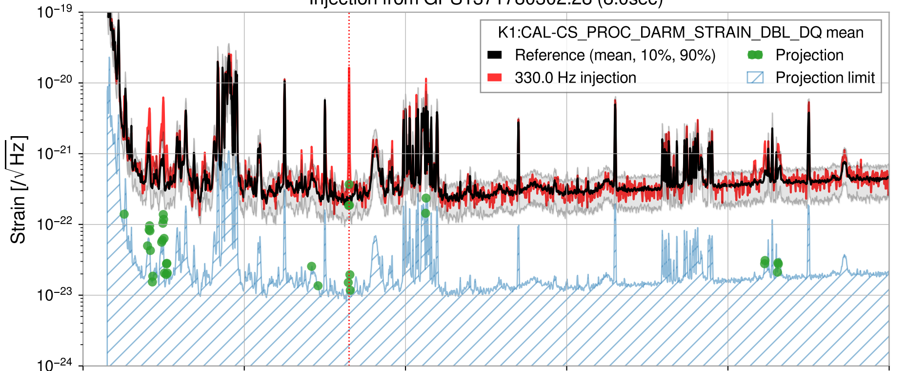
Injection from GPS1371780302.28 (8.0sec)
