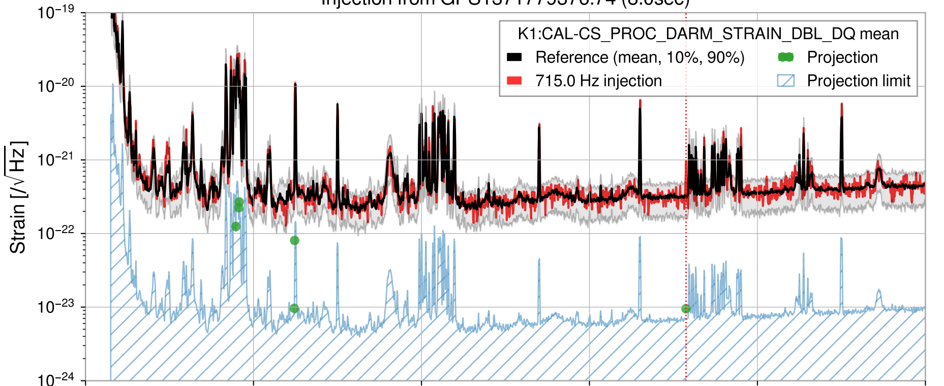
Injection from GPS1371779376.74 (8.0sec)
