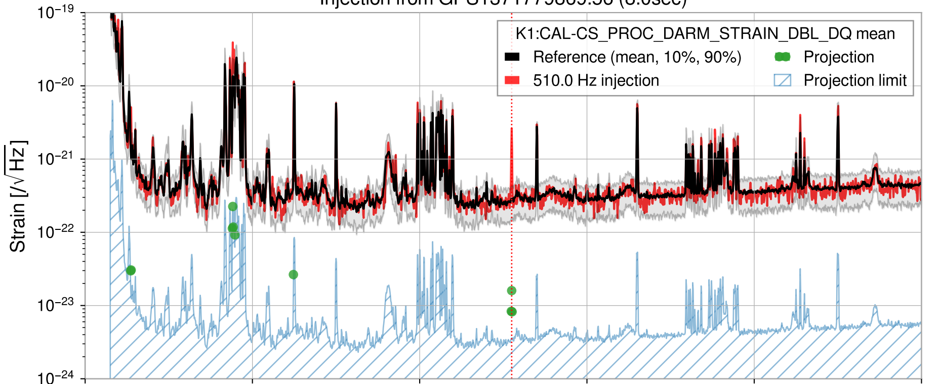
Injection from GPS1371779869.56 (8.0sec)
