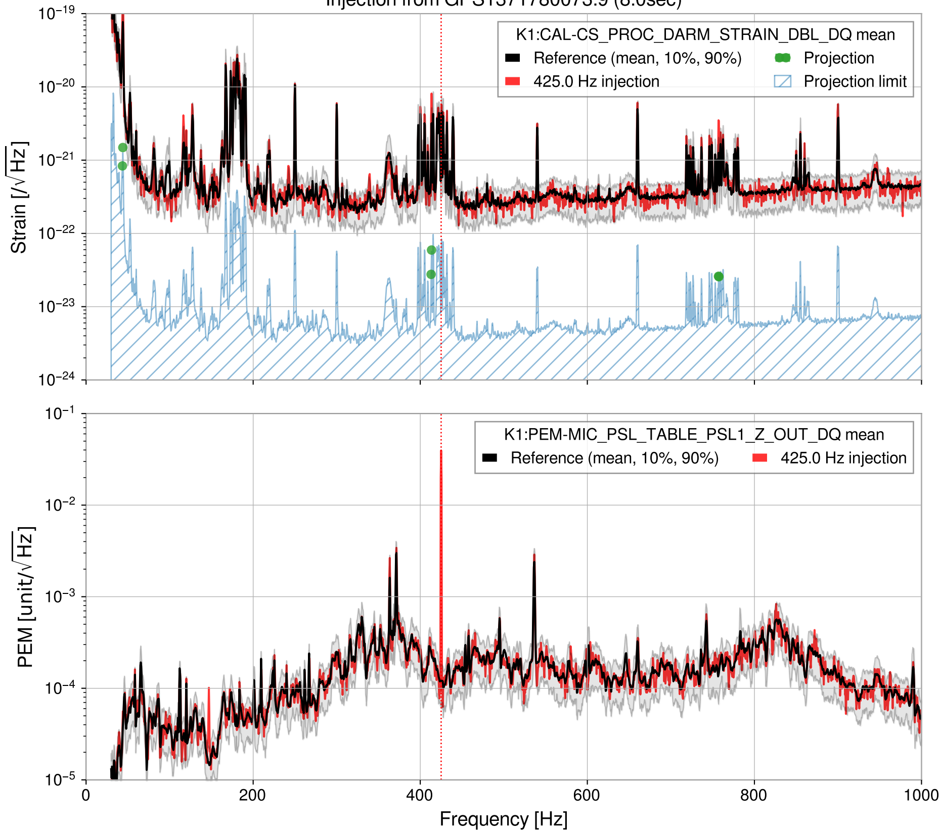
Injection from GPS1371780073.9 (8.0sec)
