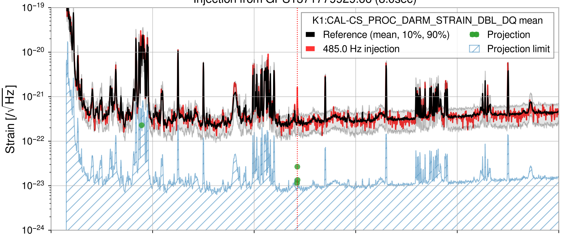
Injection from GPS1371779929.66 (8.0sec)
