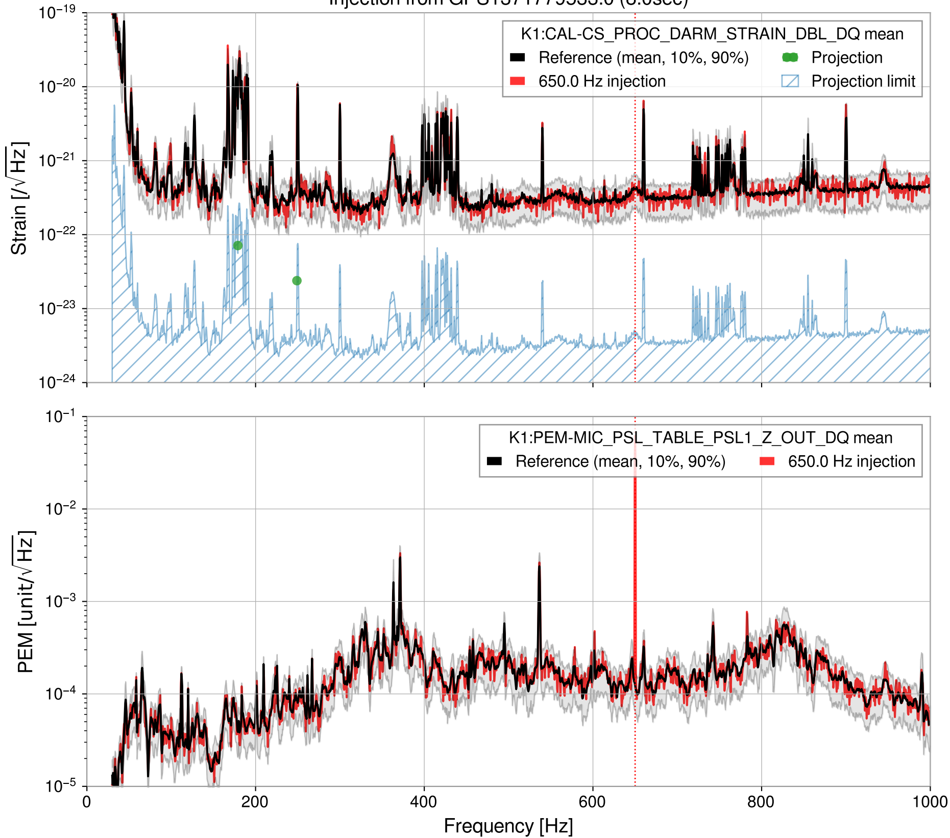
Injection from GPS1371779533.0 (8.0sec)
