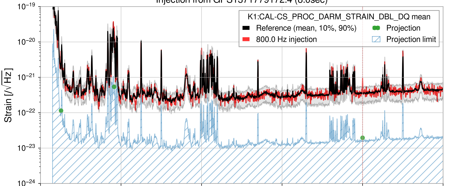
Injection from GPS1371779172.4 (8.0sec)
