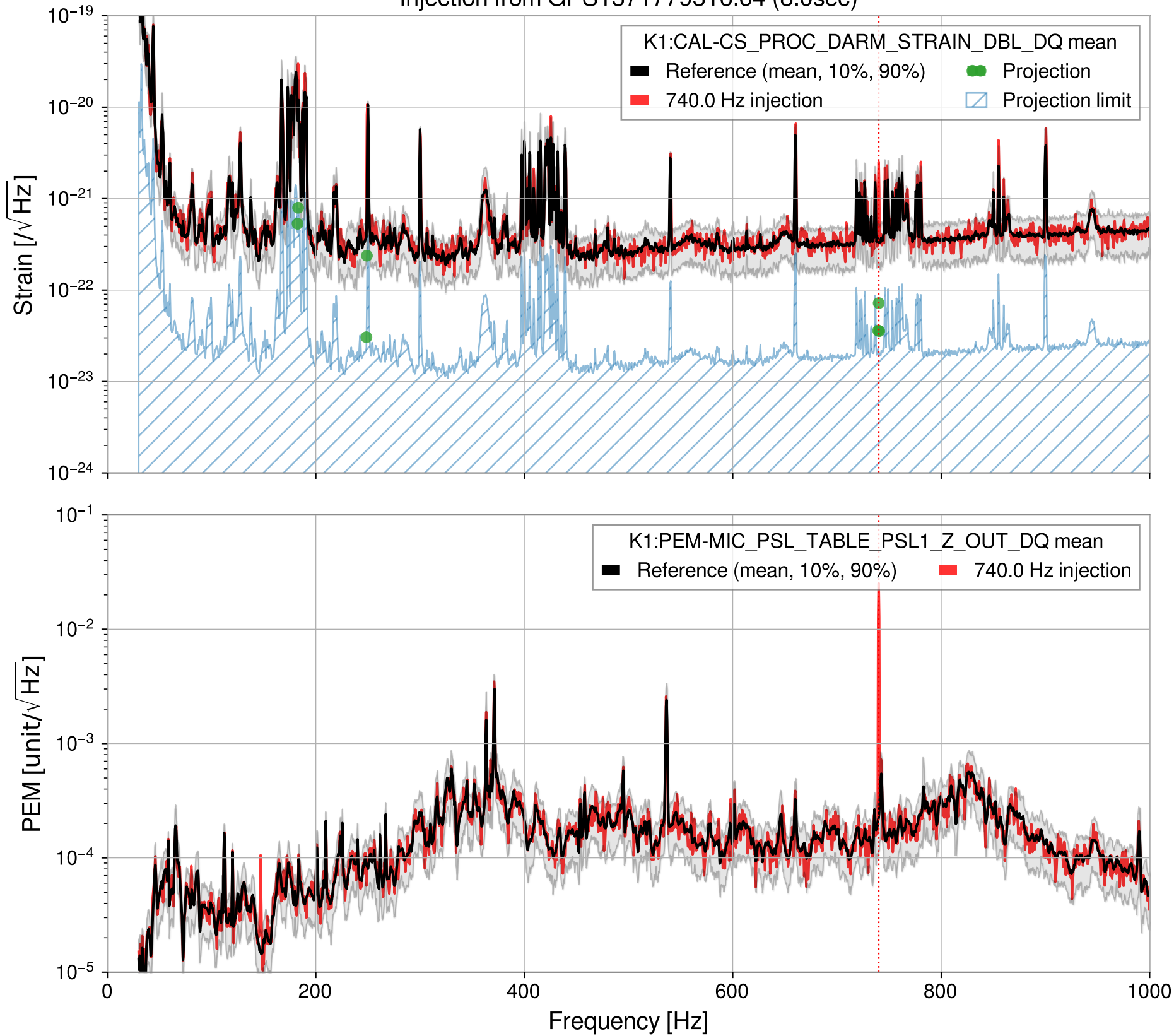
Injection from GPS1371779316.64 (8.0sec)
