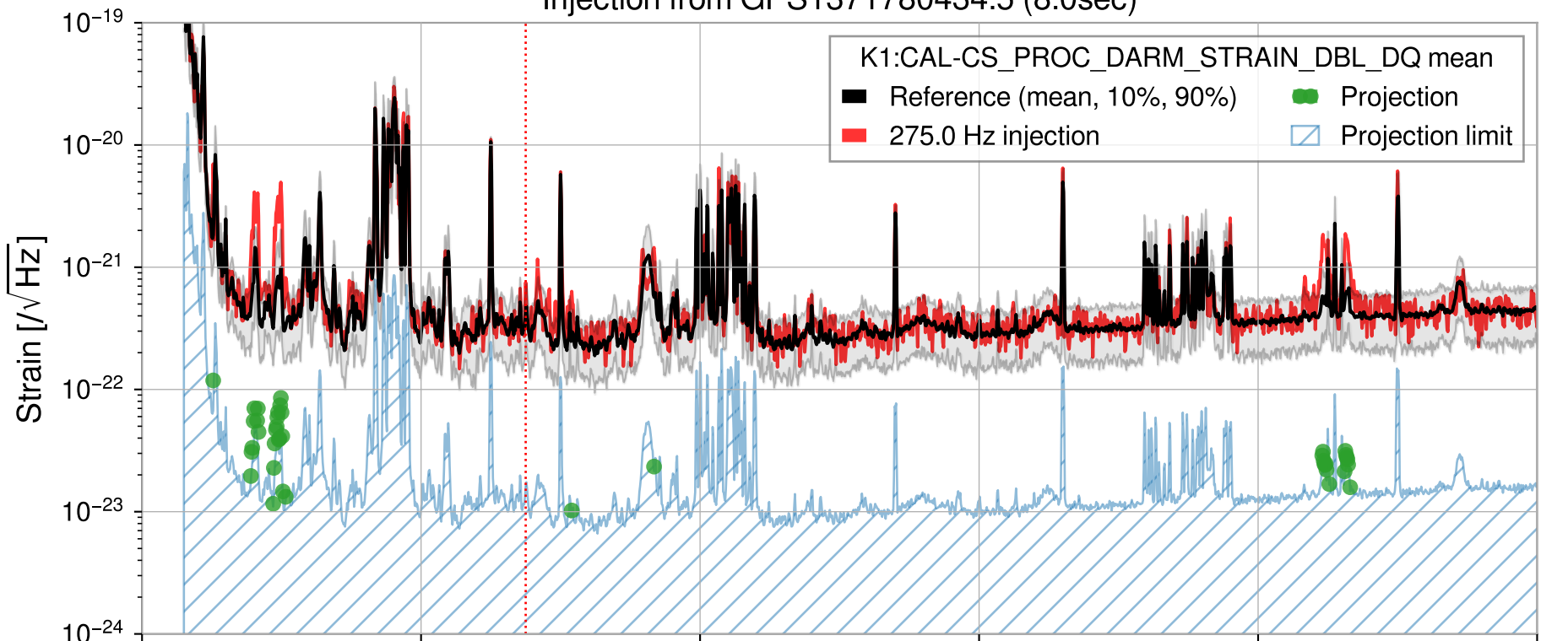
Injection from GPS1371780434.5 (8.0sec)
