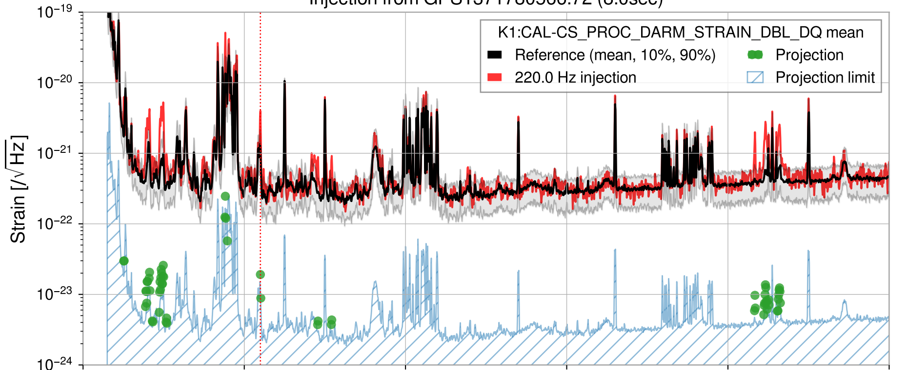
Injection from GPS1371780566.72 (8.0sec)
