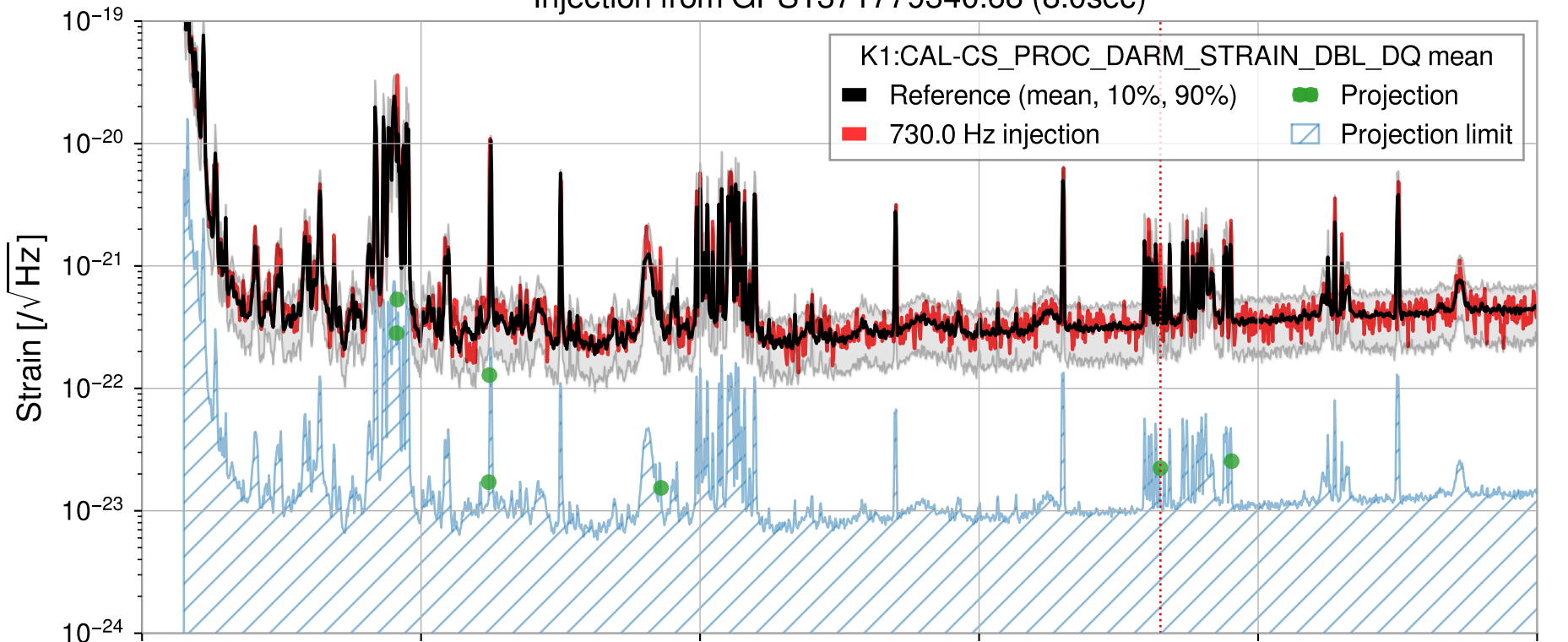
Injection from GPS1371779340.68 (8.0sec)
