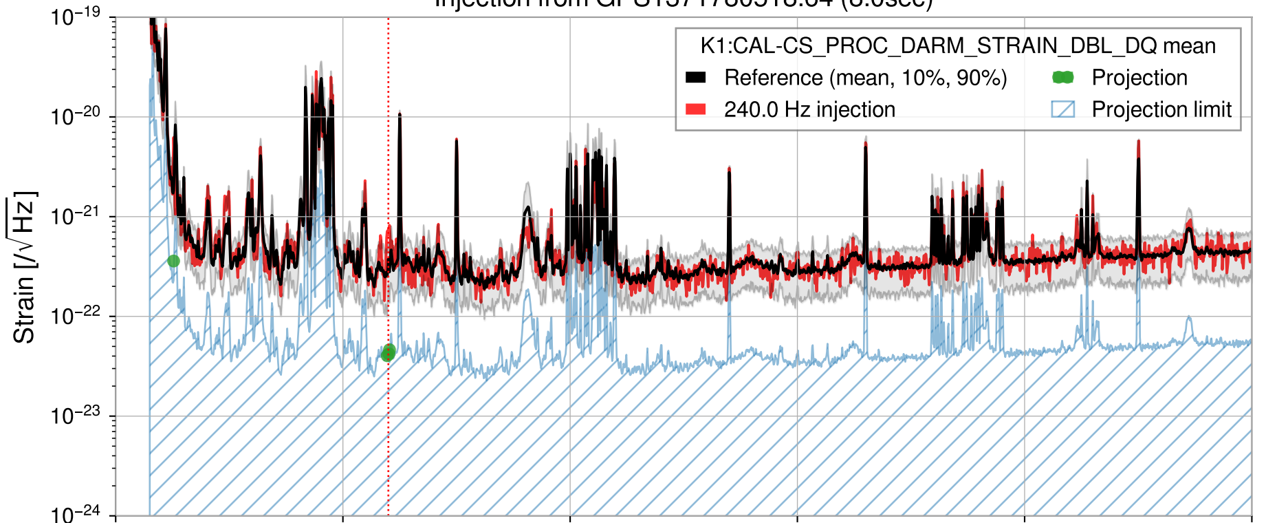
Injection from GPS1371780518.64 (8.0sec)
