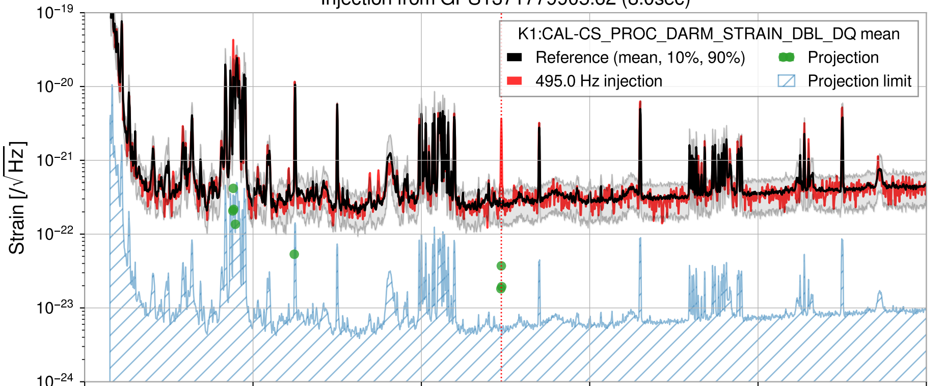
Injection from GPS1371779905.62 (8.0sec)
