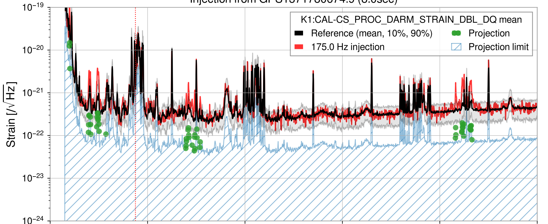
Injection from GPS1371780674.9 (8.0sec)
