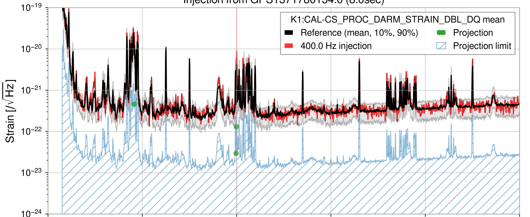
Injection from GPS1371780134.0 (8.0sec)
