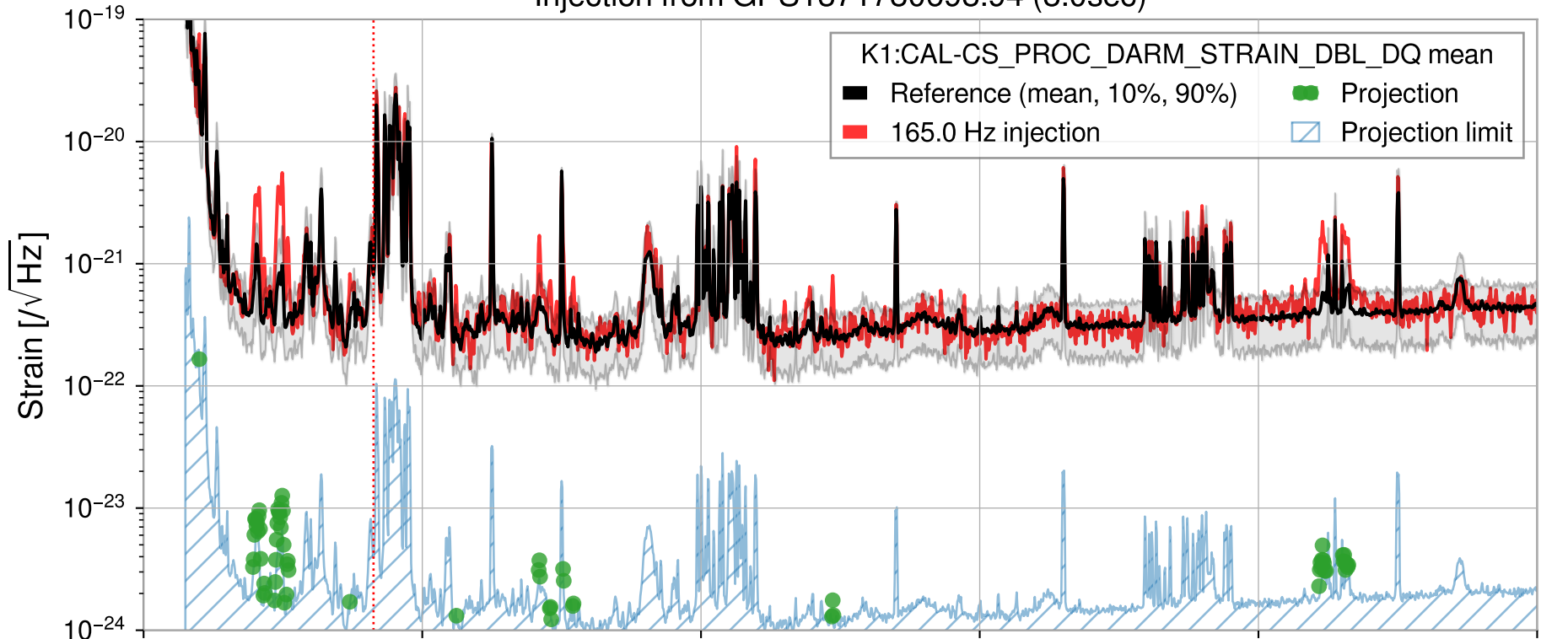
Injection from GPS1371780698.94 (8.0sec)
