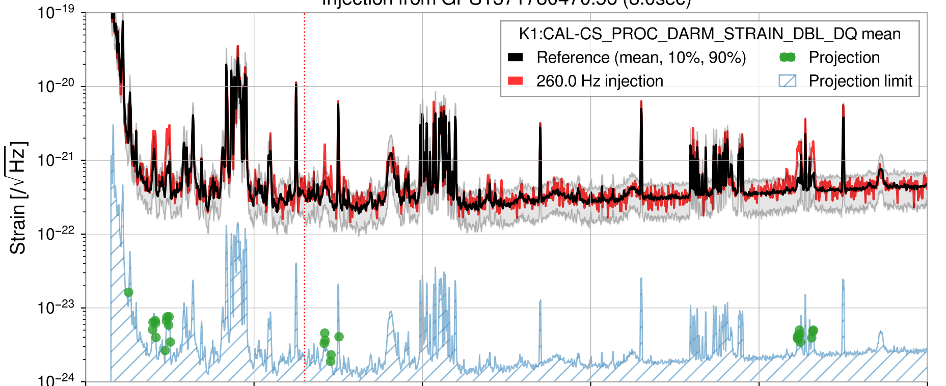
Injection from GPS1371780470.56 (8.0sec)
