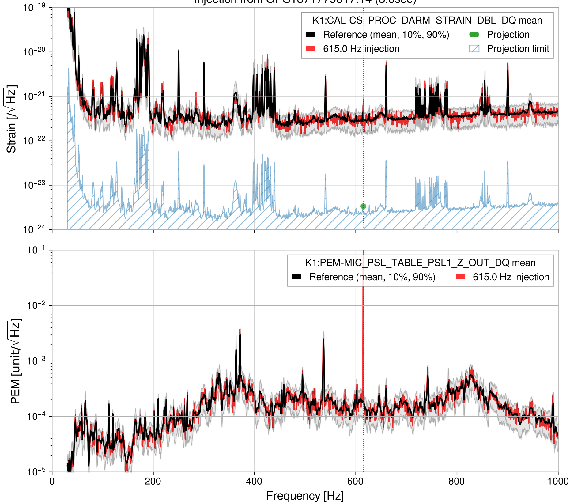
Injection from GPS1371779617.14 (8.0sec)
