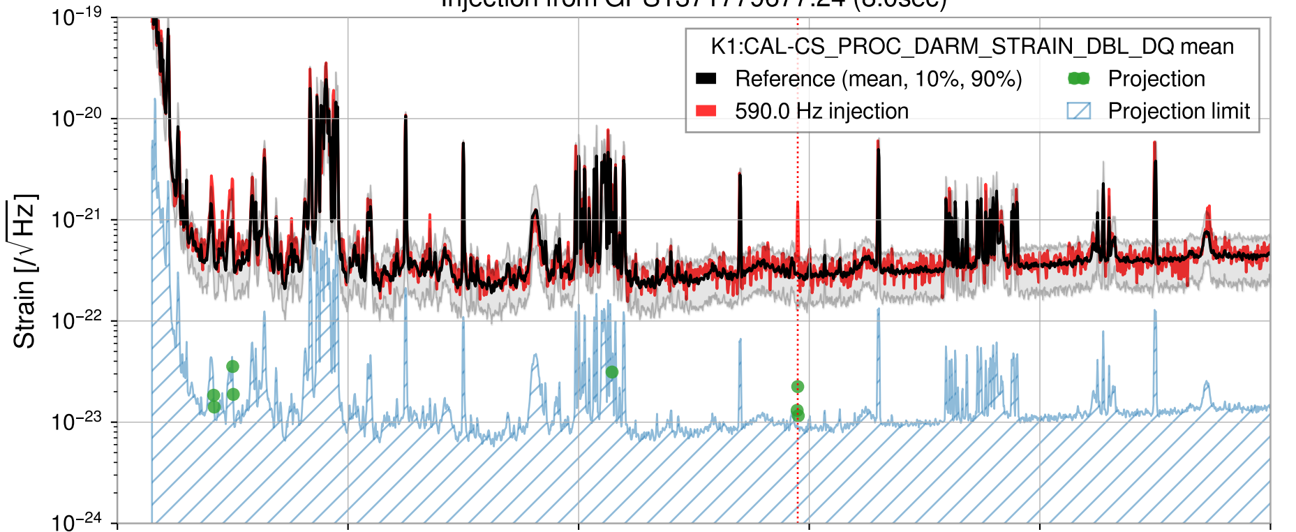
Injection from GPS1371779677.24 (8.0sec)
