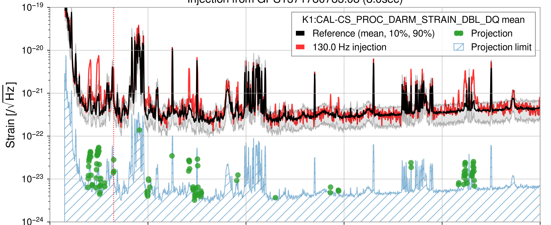
Injection from GPS1371780783.08 (8.0sec)
