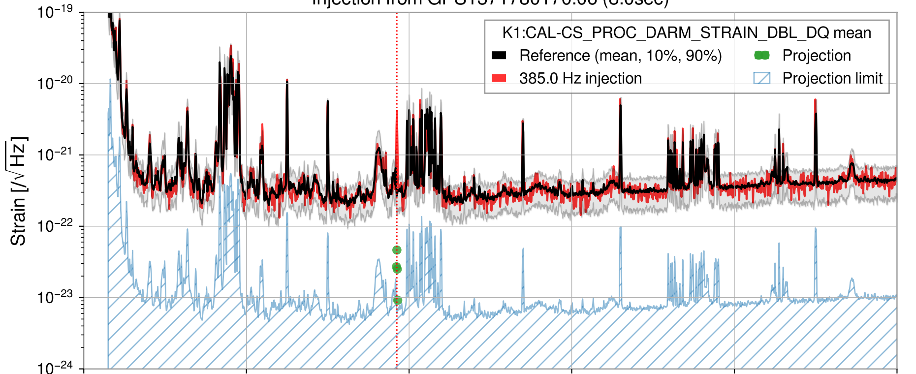
Injection from GPS1371780170.06 (8.0sec)
