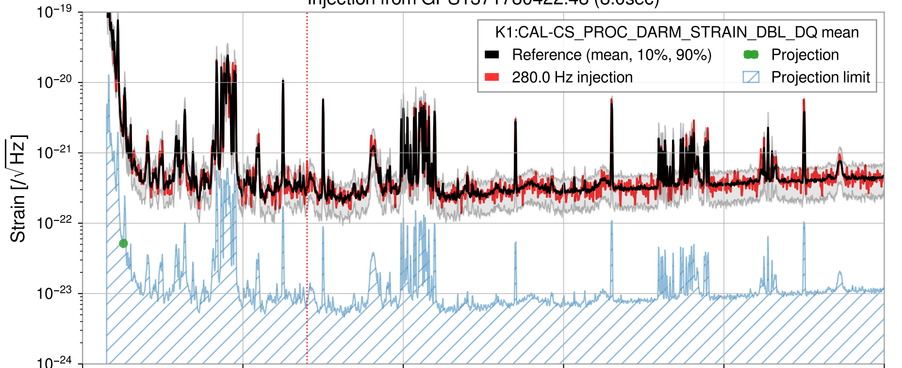
Injection from GPS1371780422.48 (8.0sec)
