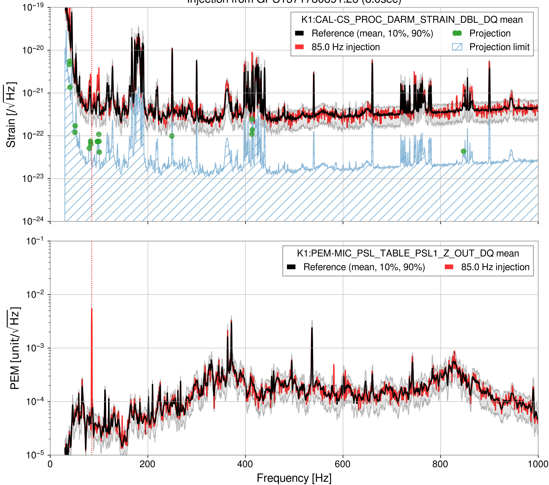
Injection from GPS1371780891.26 (8.0sec)
