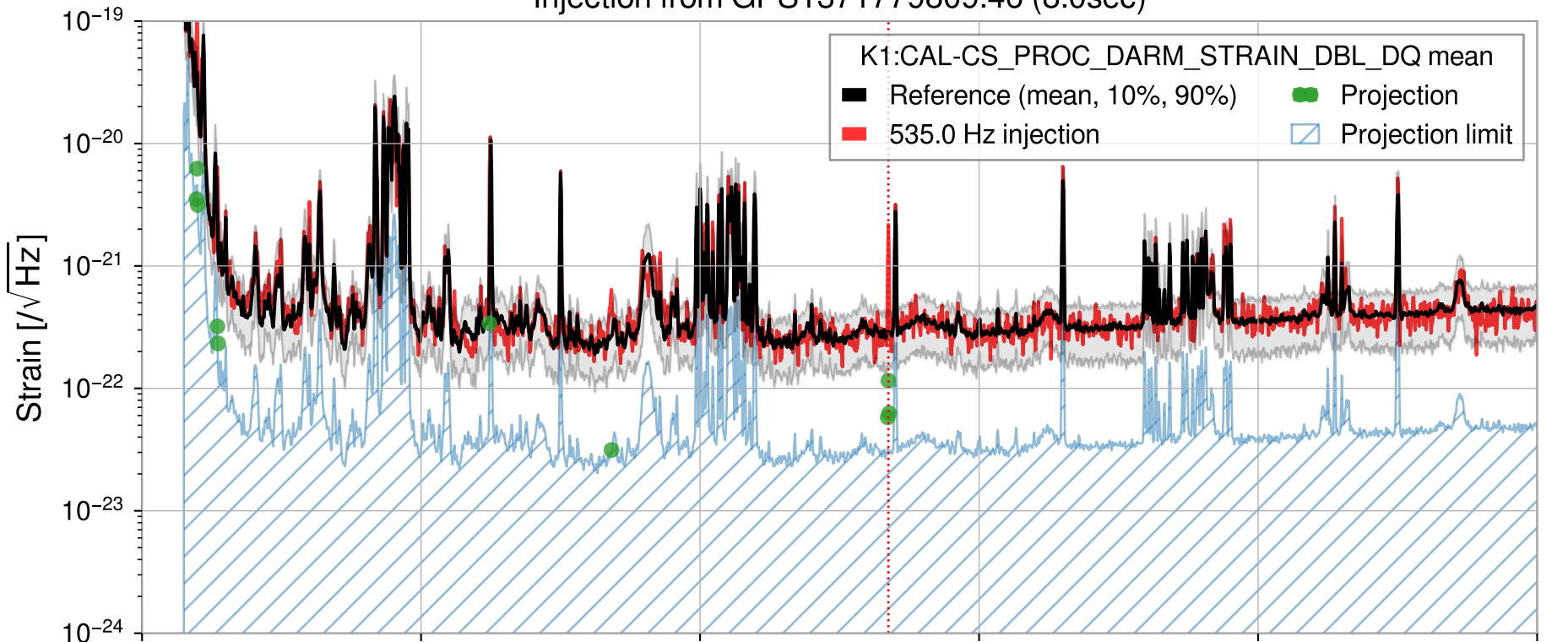
Injection from GPS1371779809.46 (8.0sec)
