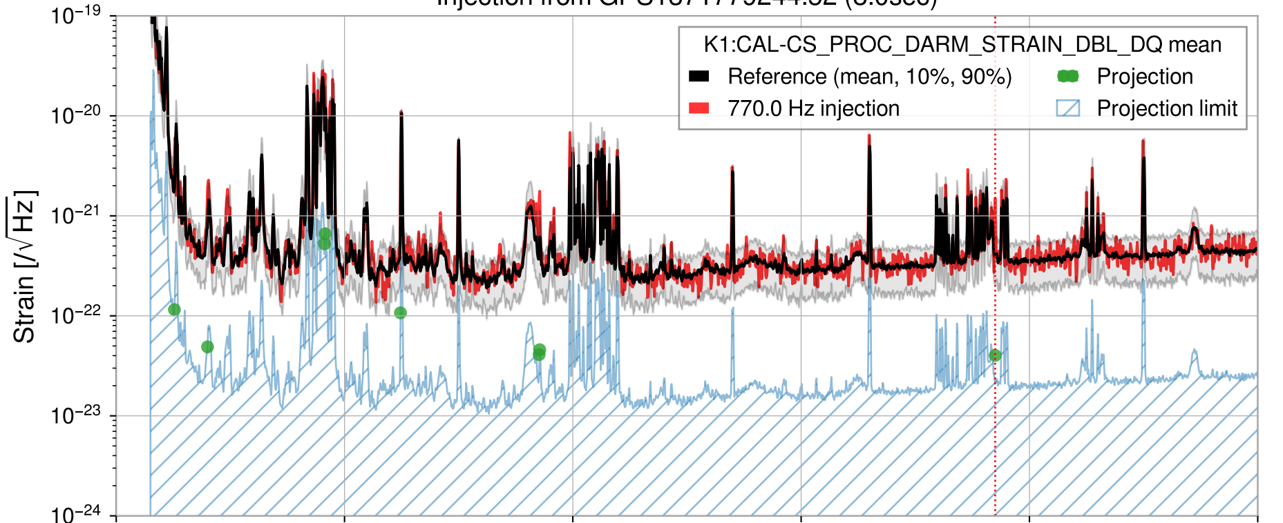
Injection from GPS1371779244.52 (8.0sec)
