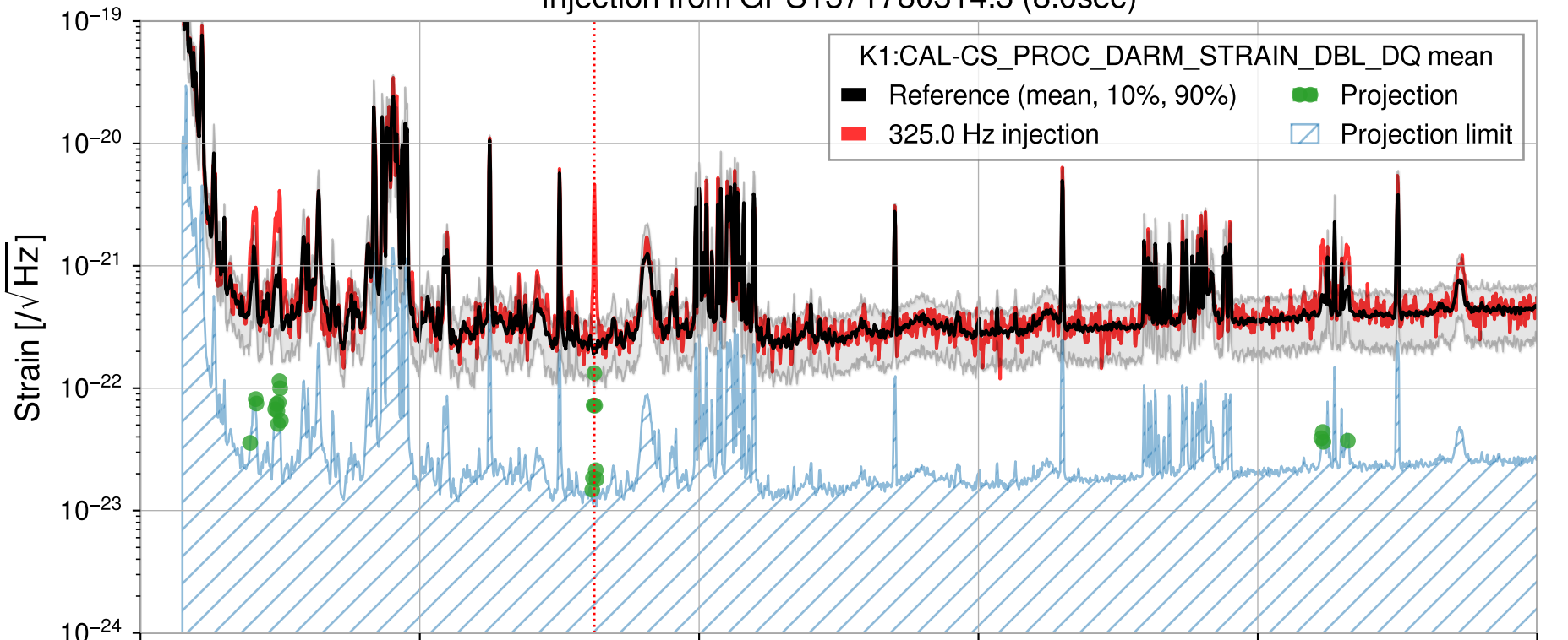
Injection from GPS1371780314.3 (8.0sec)
