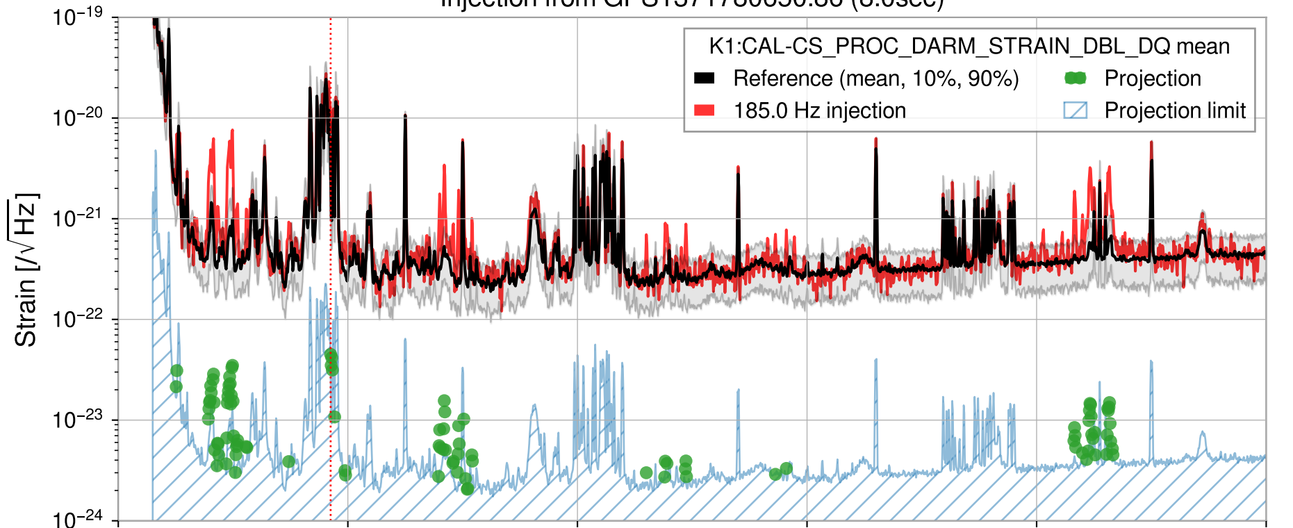
Injection from GPS1371780650.86 (8.0sec)
