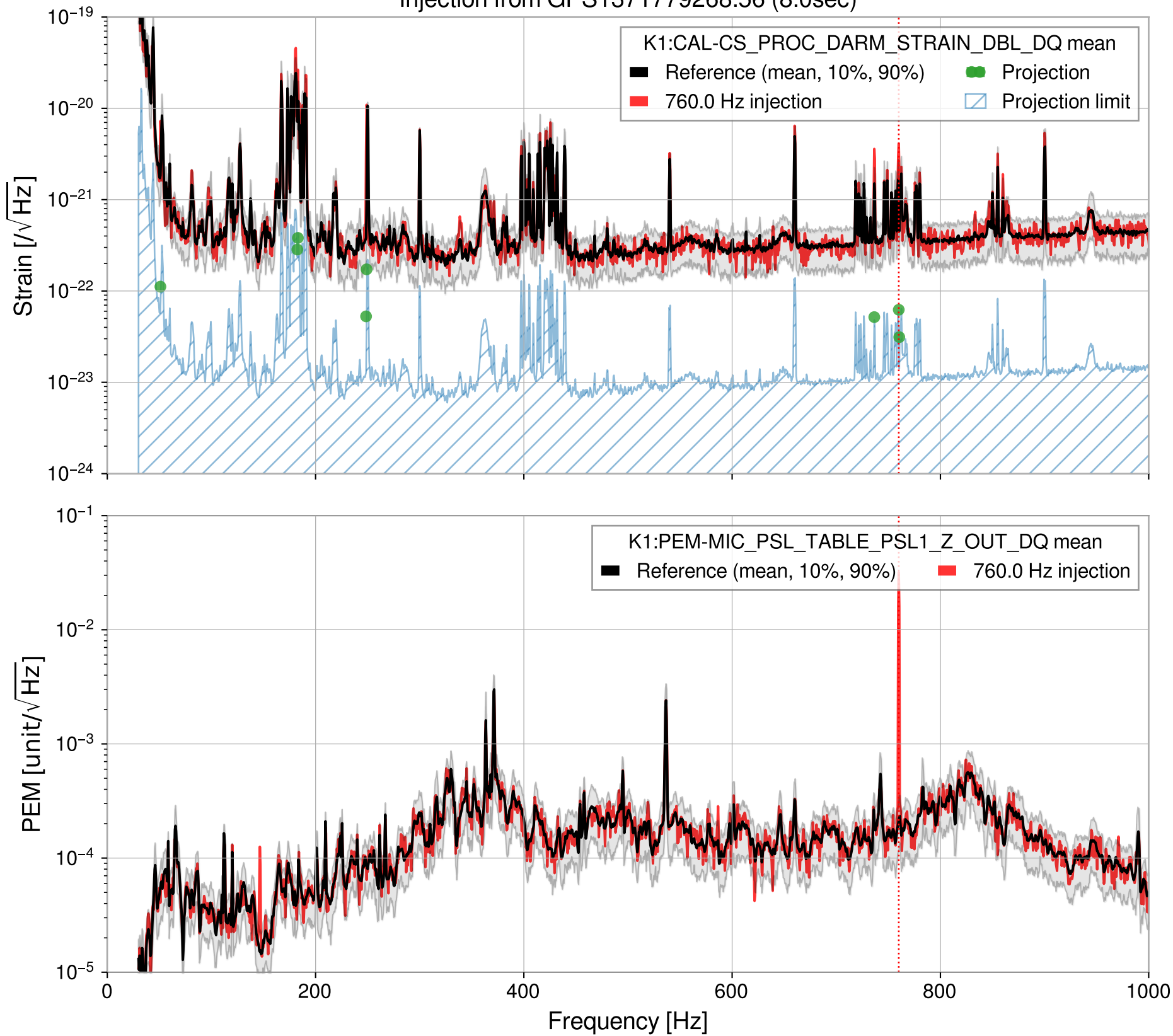
Injection from GPS1371779268.56 (8.0sec)
