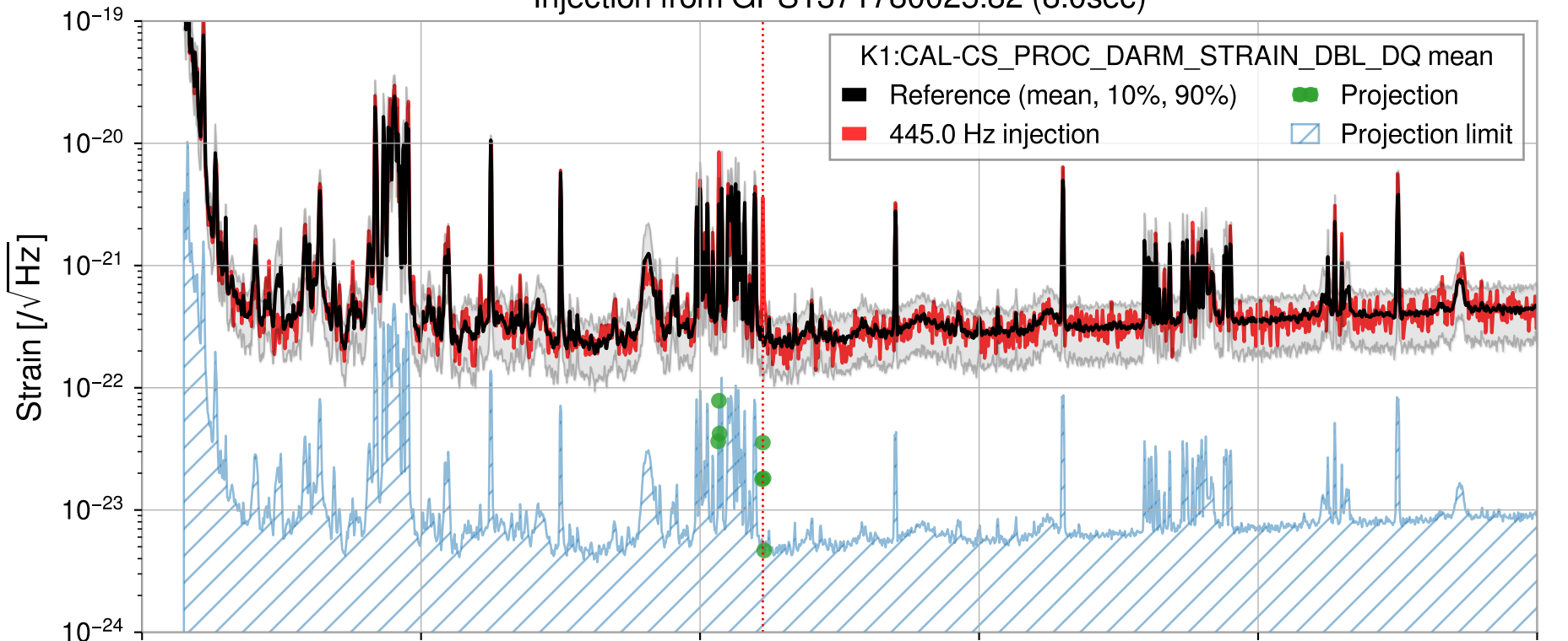
Injection from GPS1371780025.82 (8.0sec)
