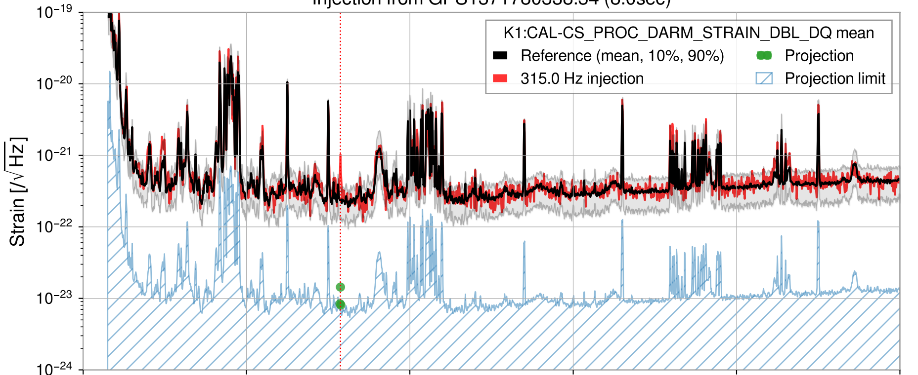
Injection from GPS1371780338.34 (8.0sec)
