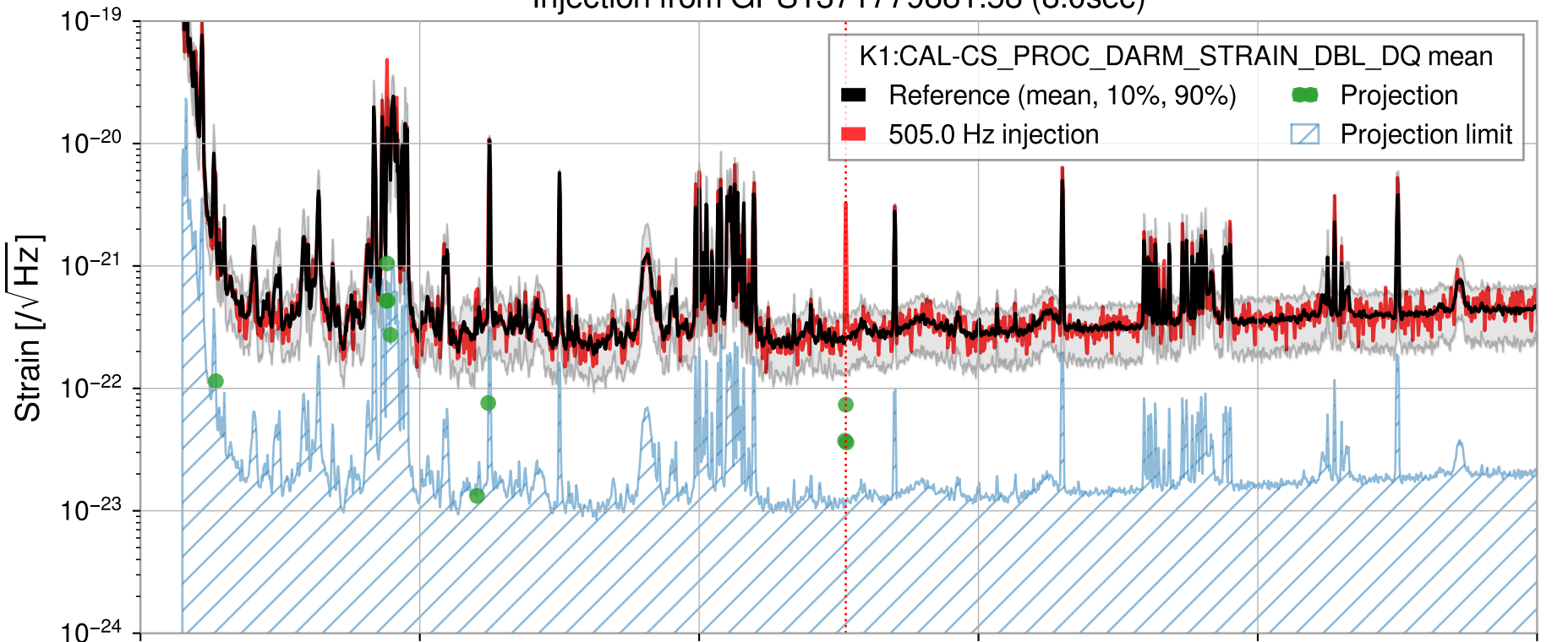
Injection from GPS1371779881.58 (8.0sec)
