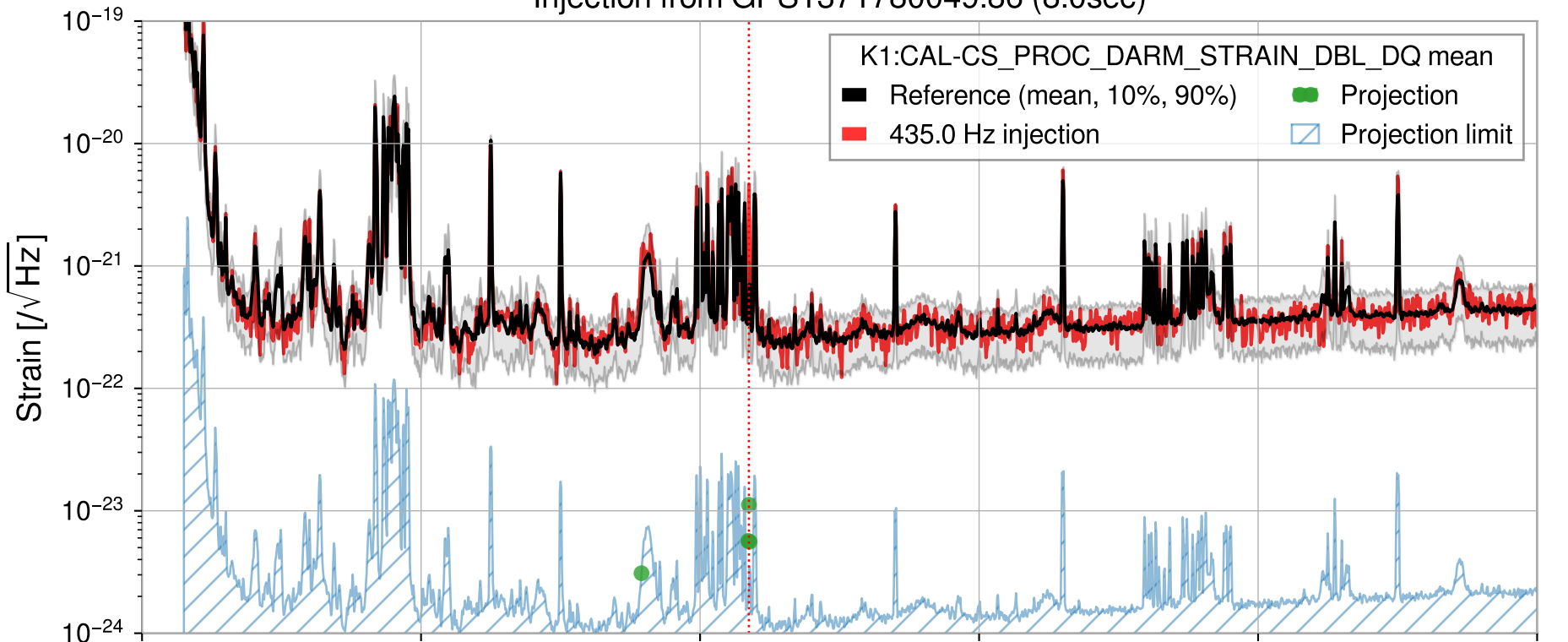
Injection from GPS1371780049.86 (8.0sec)
