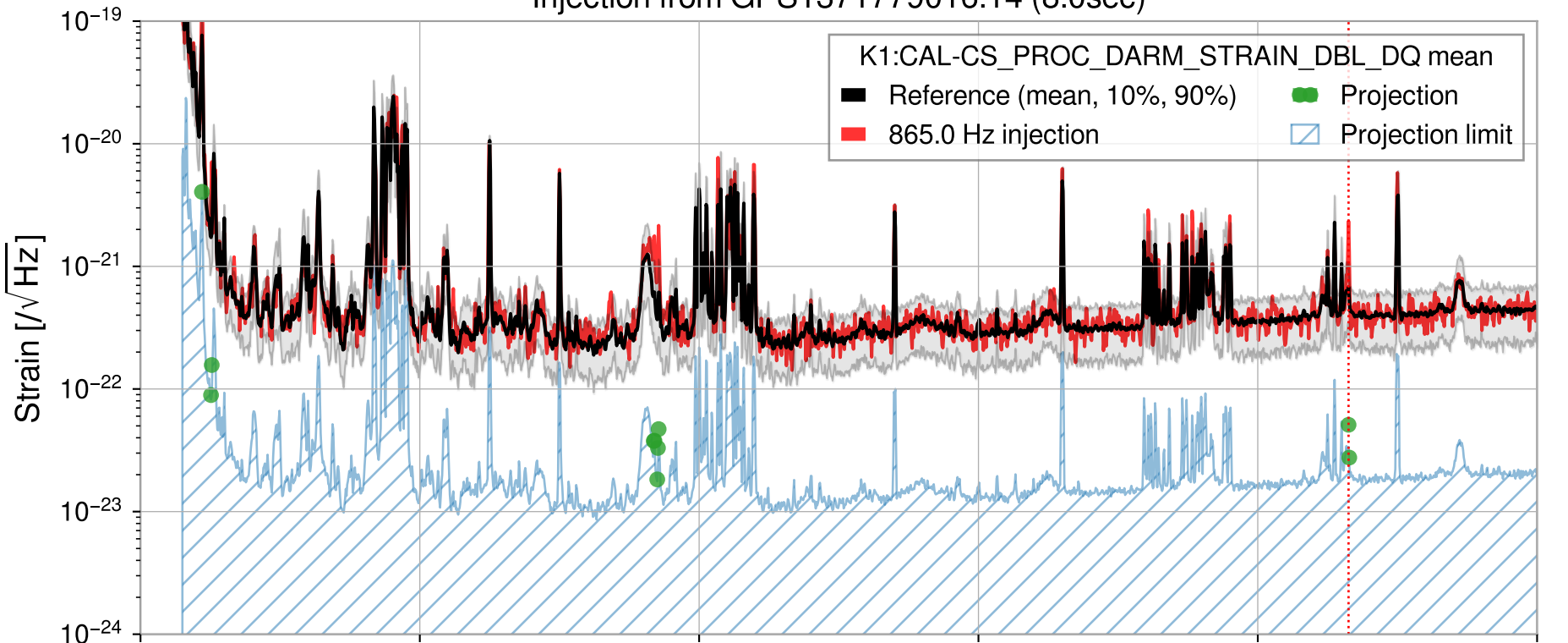
Injection from GPS1371779016.14 (8.0sec)
