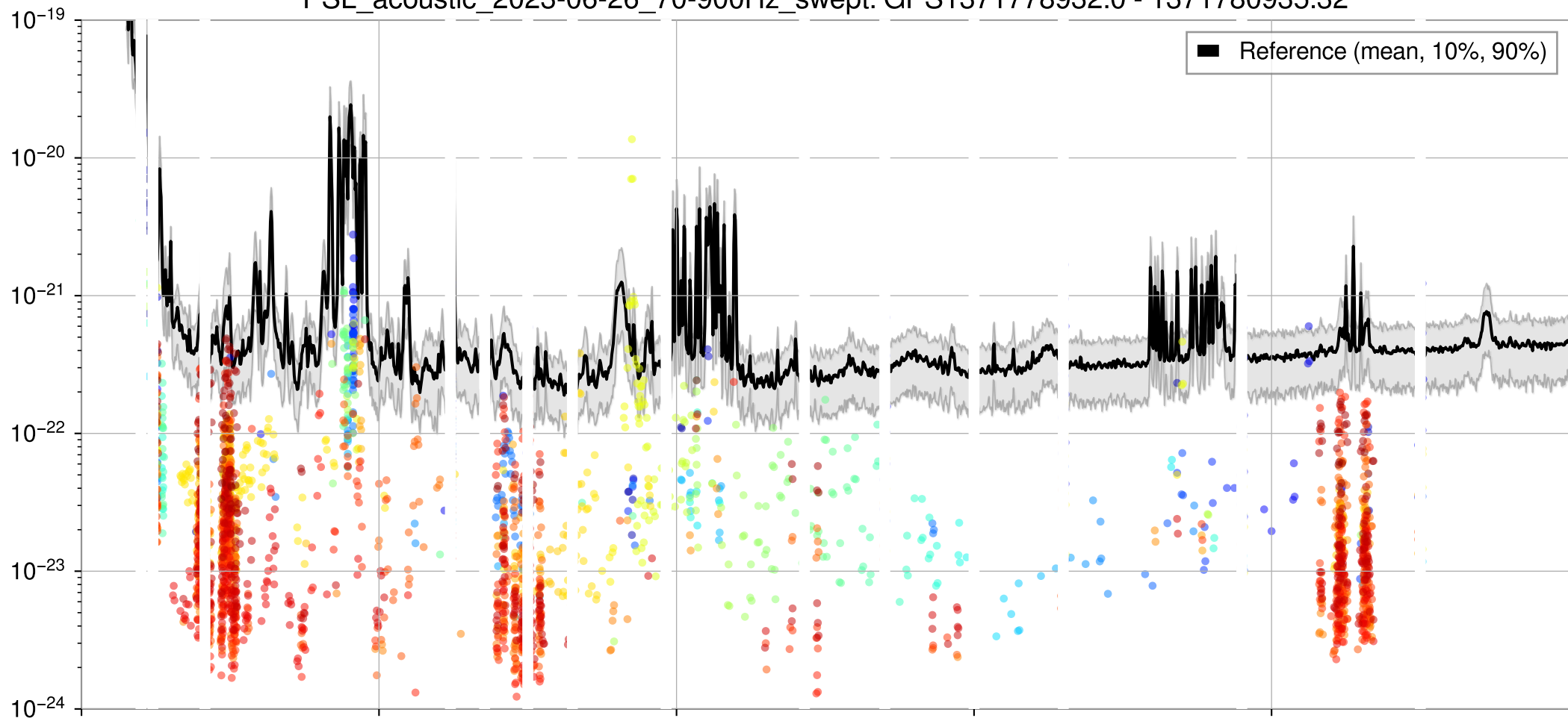
PSL_acoustic_2023-06-26_70-900Hz_swept: GPS1371778932.0 - 1371780935.32
