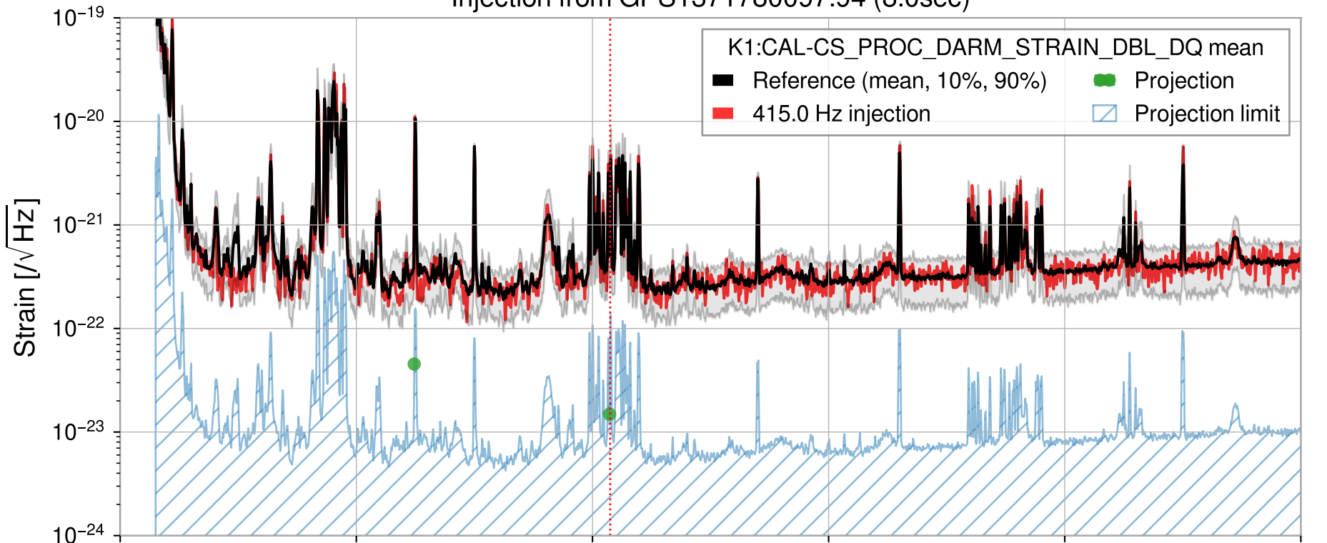
Injection from GPS1371780097.94 (8.0sec)
