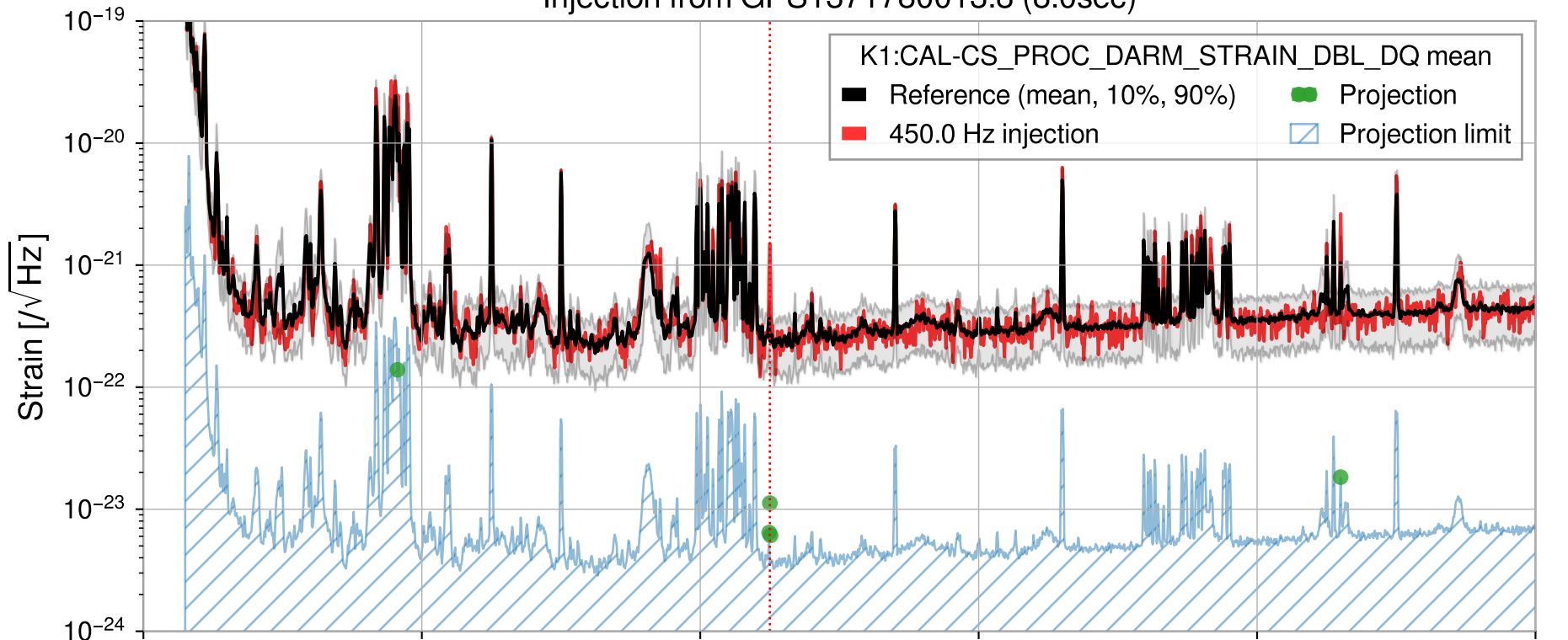
Injection from GPS1371780013.8 (8.0sec)
