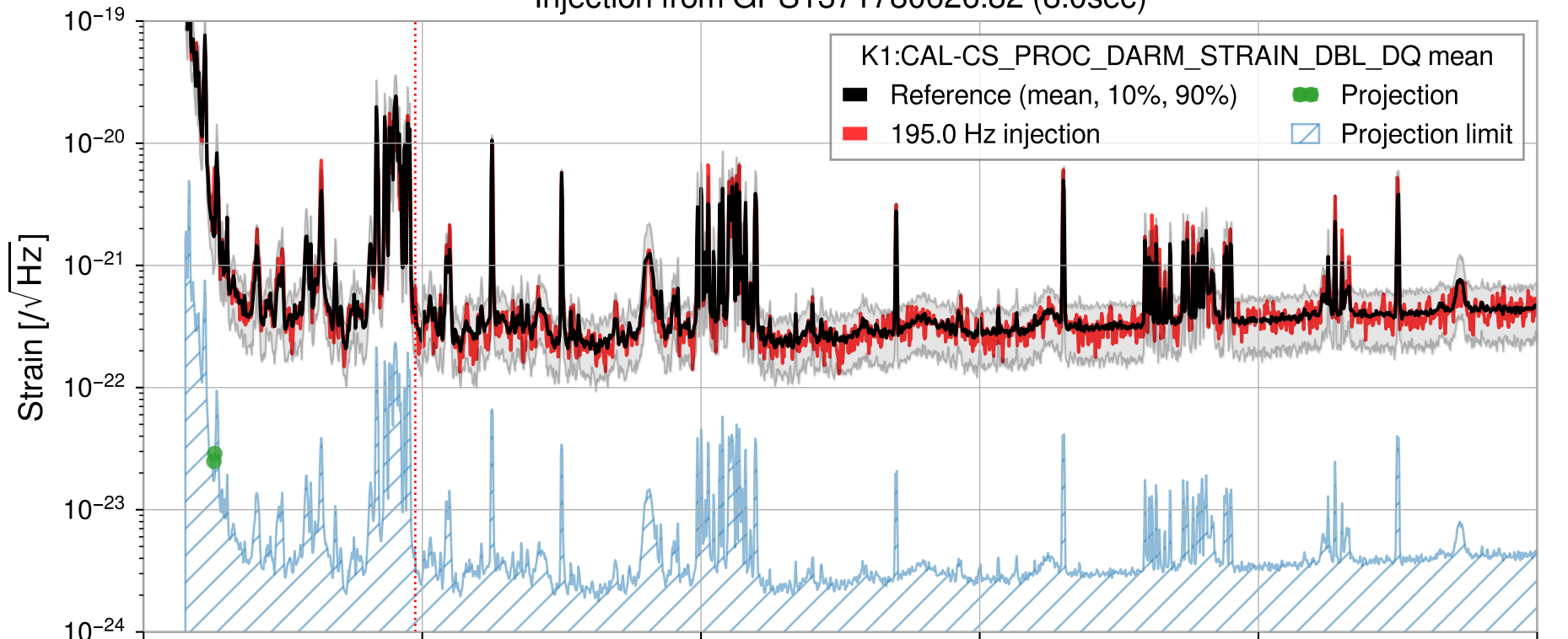
Injection from GPS1371780626.82 (8.0sec)
