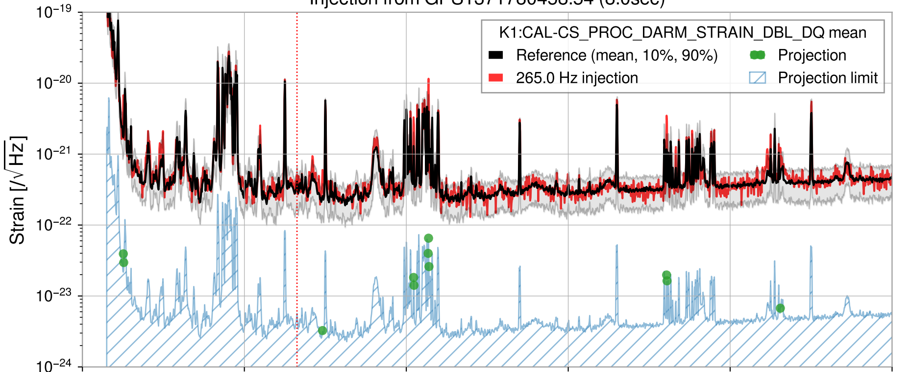
Injection from GPS1371780458.54 (8.0sec)
