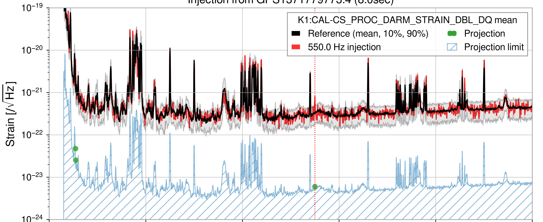
Injection from GPS1371779773.4 (8.0sec)
