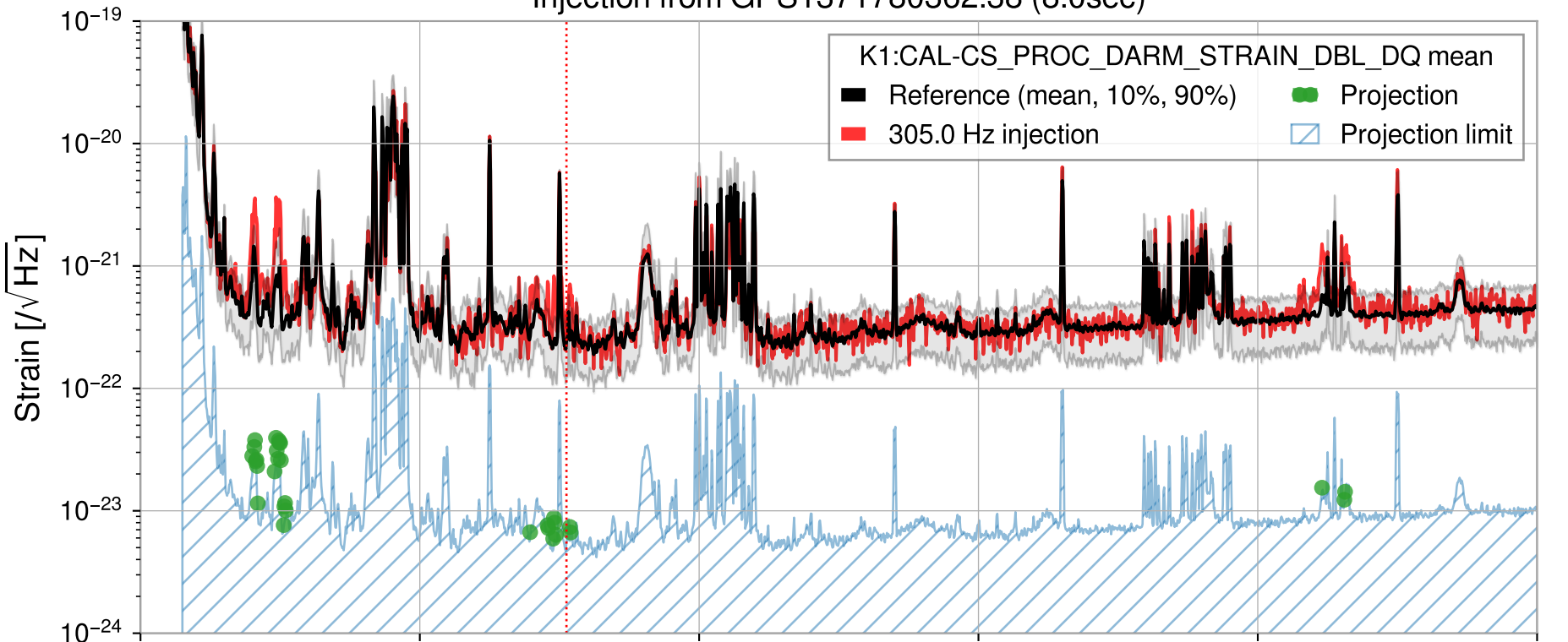
Injection from GPS1371780362.38 (8.0sec)
