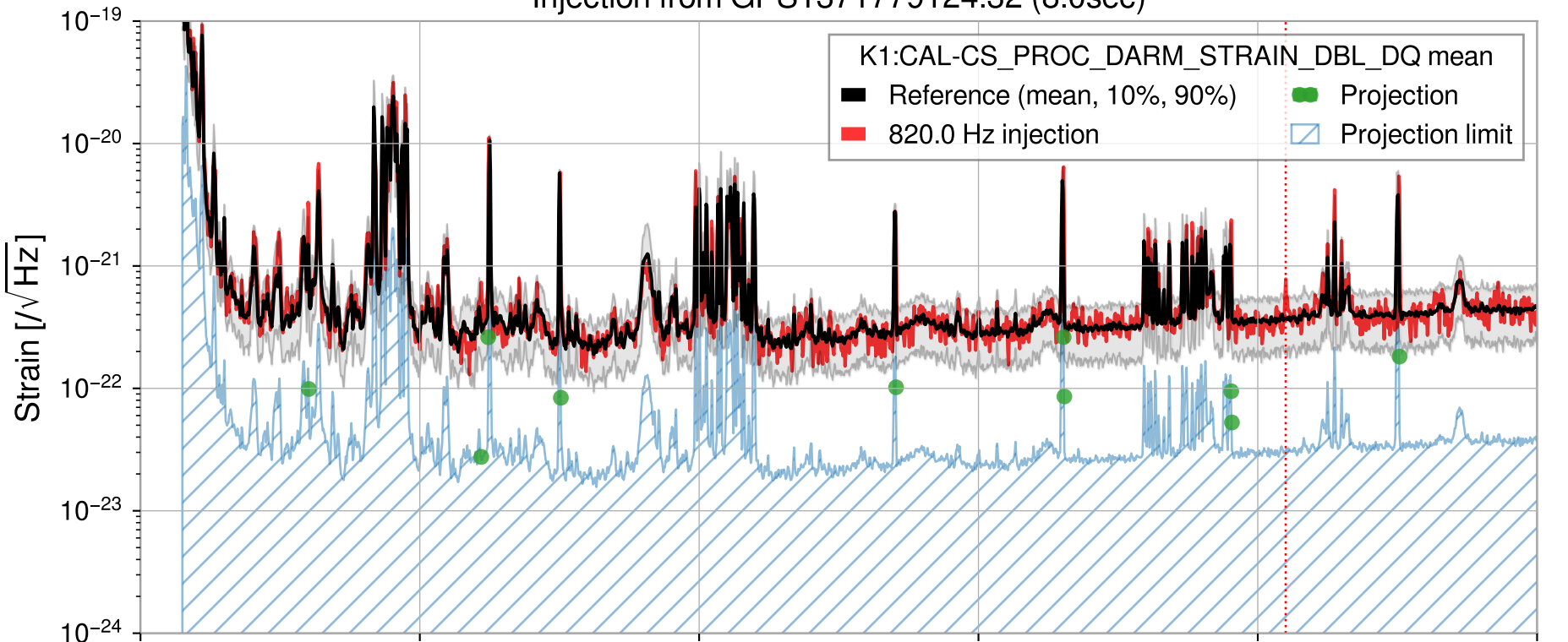
Injection from GPS1371779124.32 (8.0sec)
