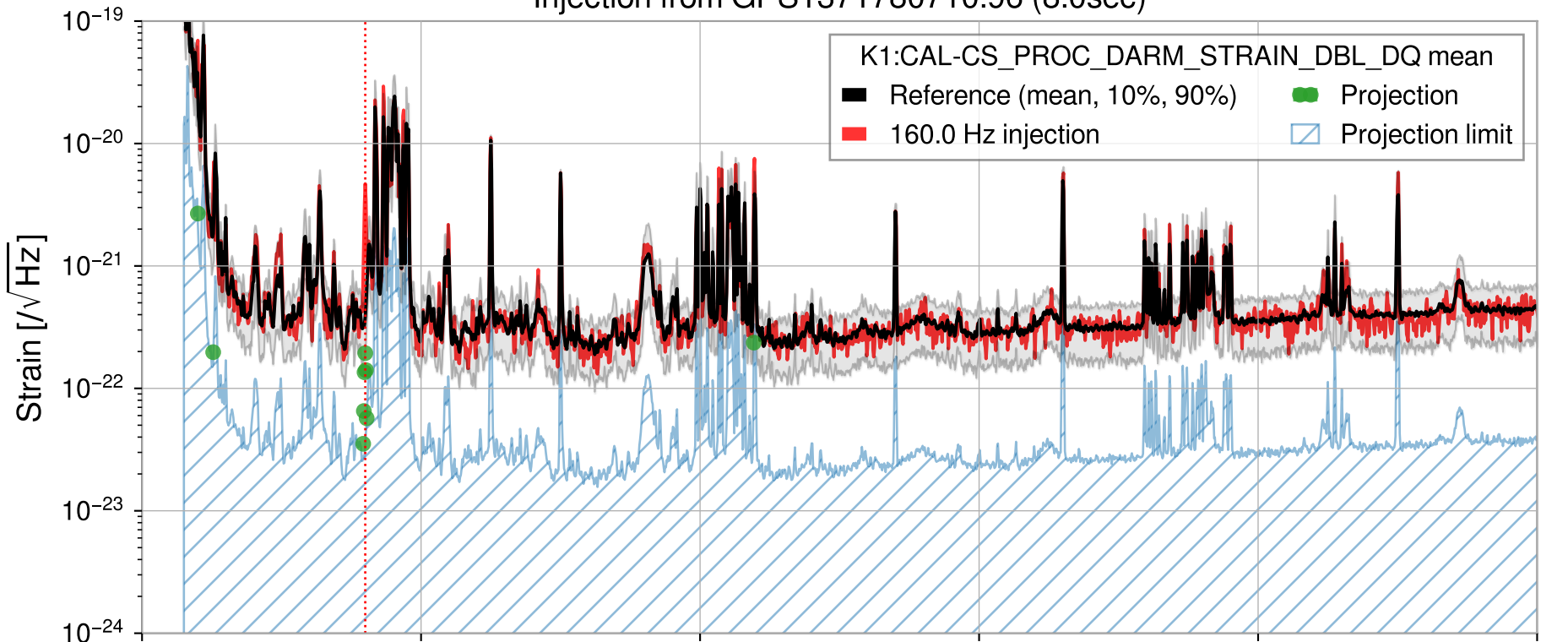
Injection from GPS1371780710.96 (8.0sec)
