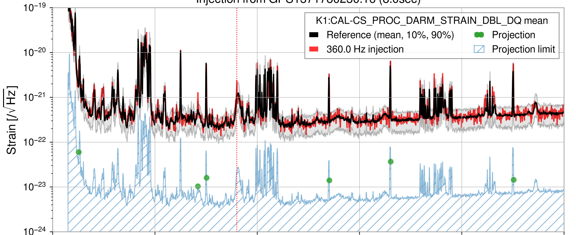
Injection from GPS1371780230.16 (8.0sec)
