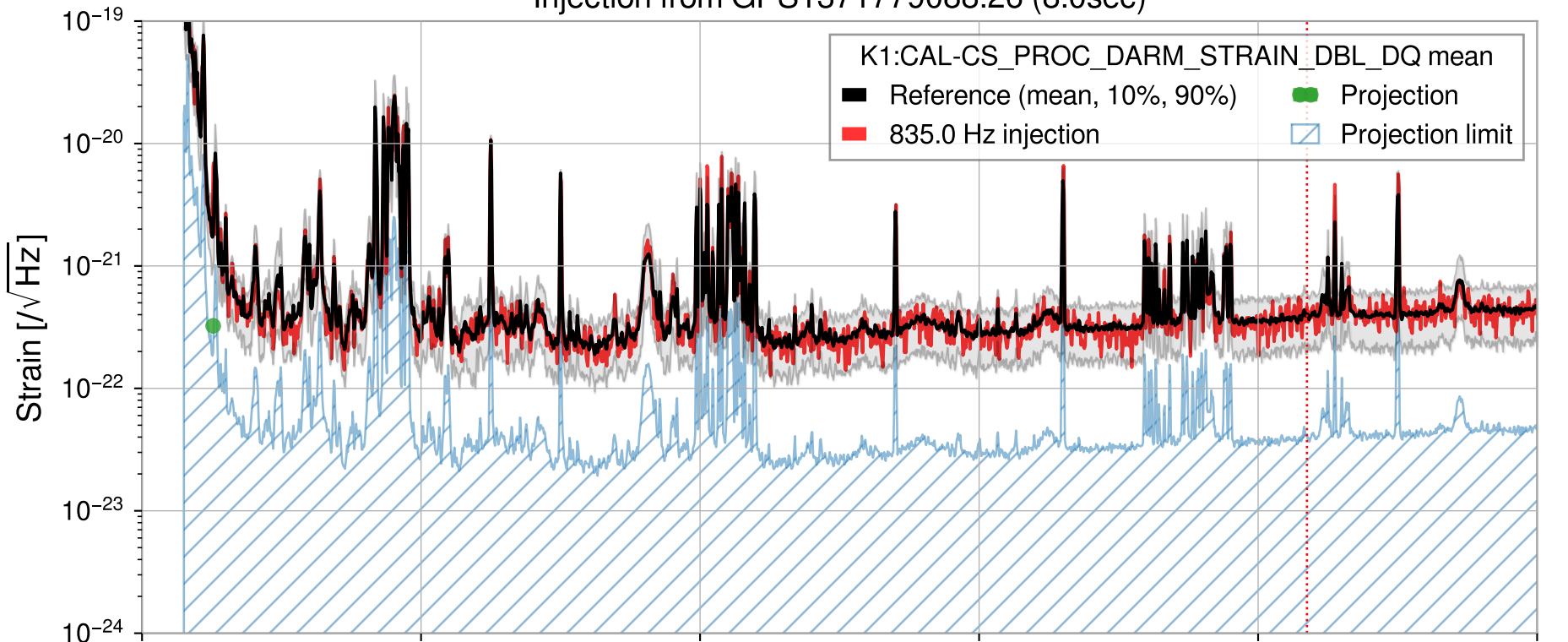
Injection from GPS1371779088.26 (8.0sec)
