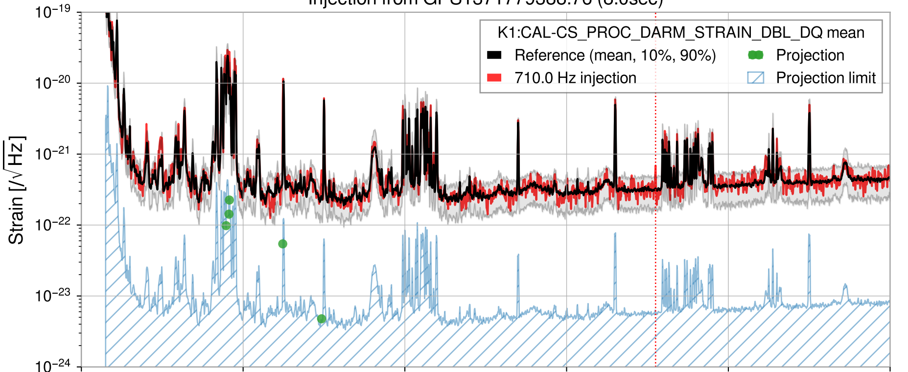
Injection from GPS1371779388.76 (8.0sec)
