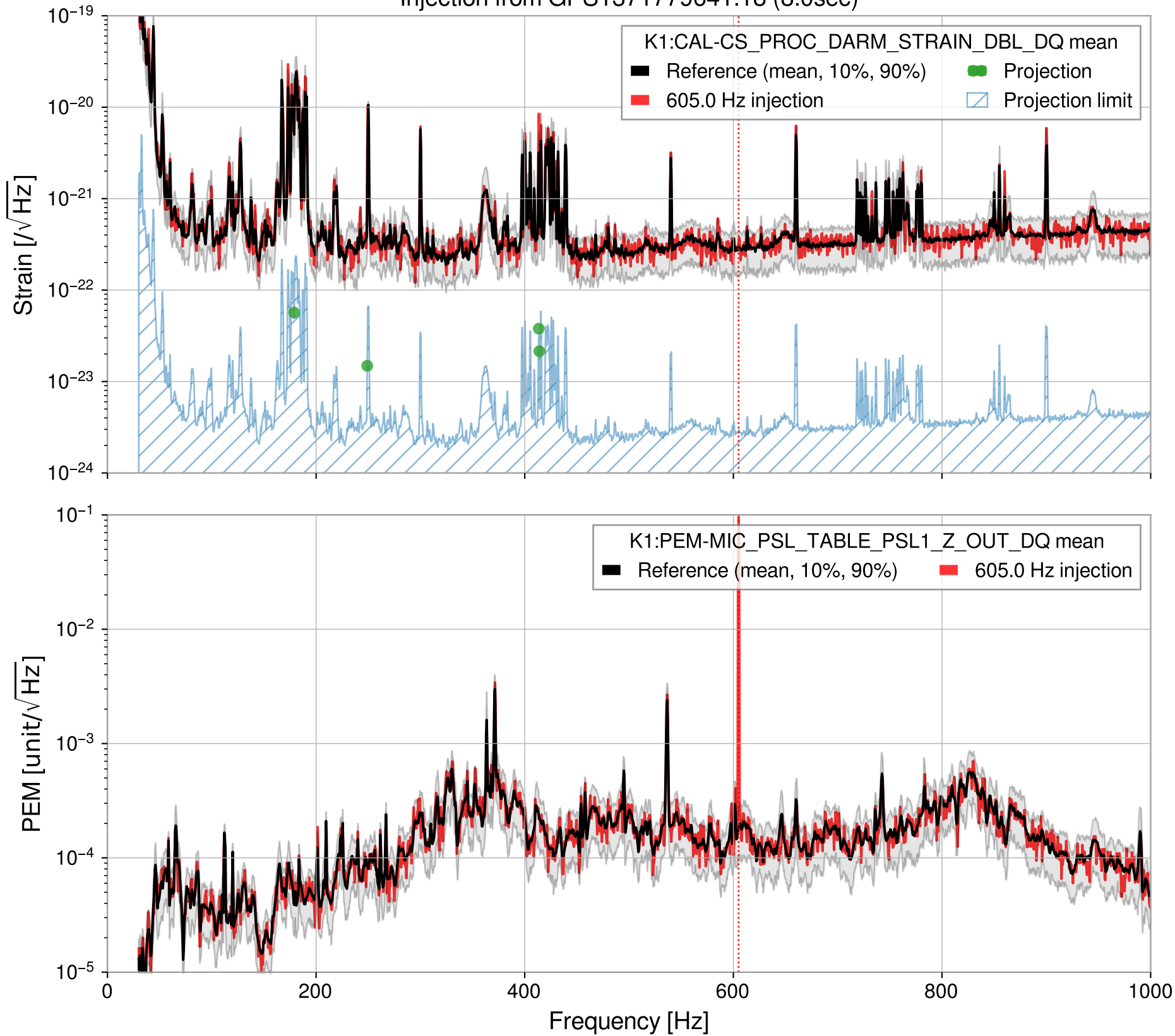
Injection from GPS1371779641.18 (8.0sec)
