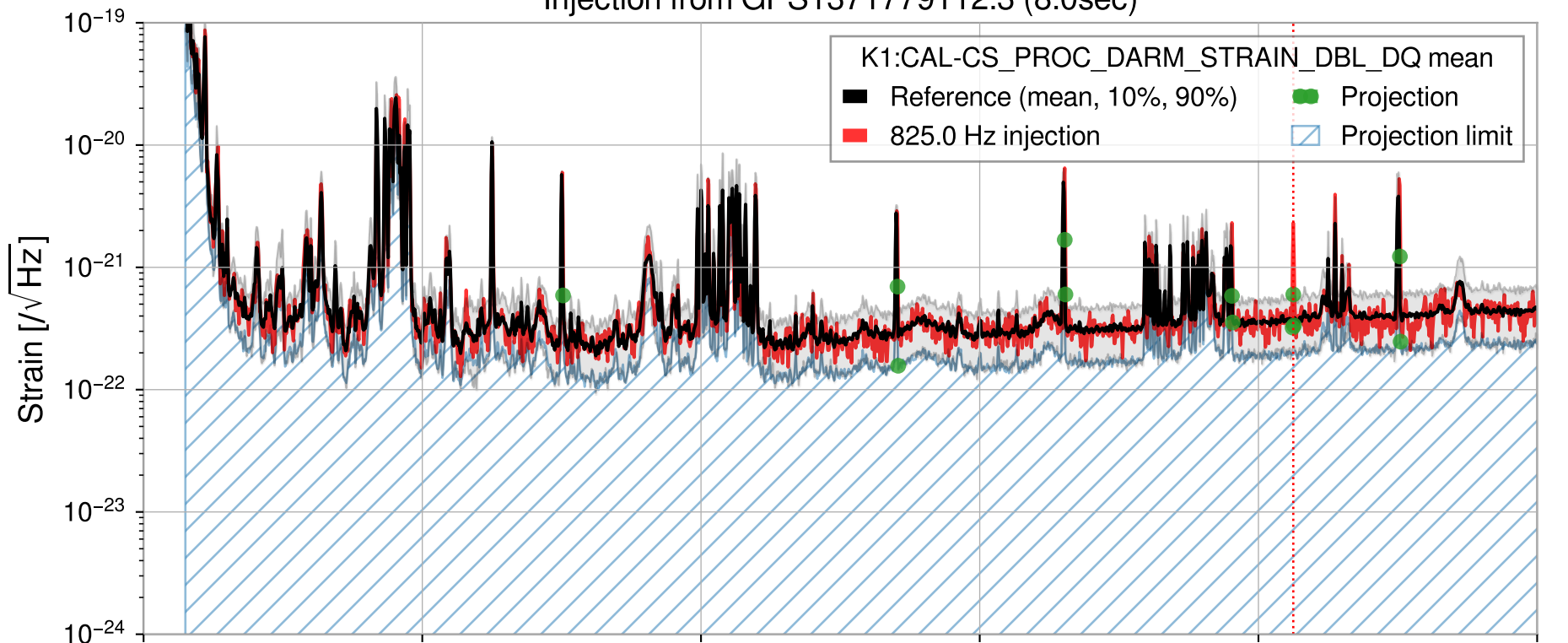
Injection from GPS1371779112.3 (8.0sec)
