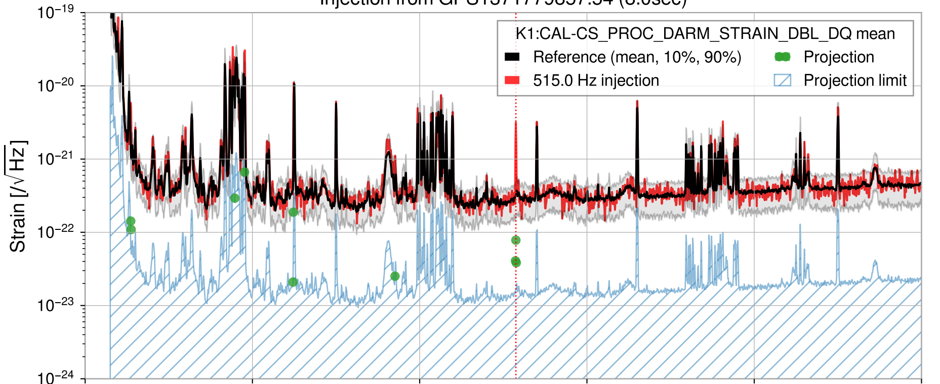
Injection from GPS1371779857.54 (8.0sec)
