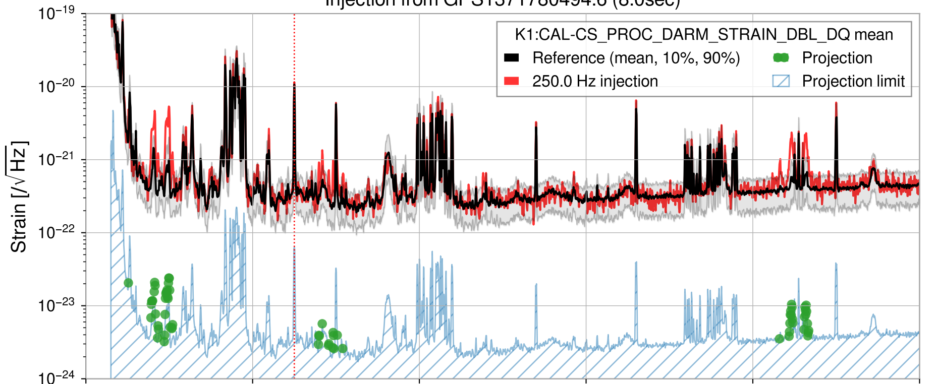
Injection from GPS1371780494.6 (8.0sec)
