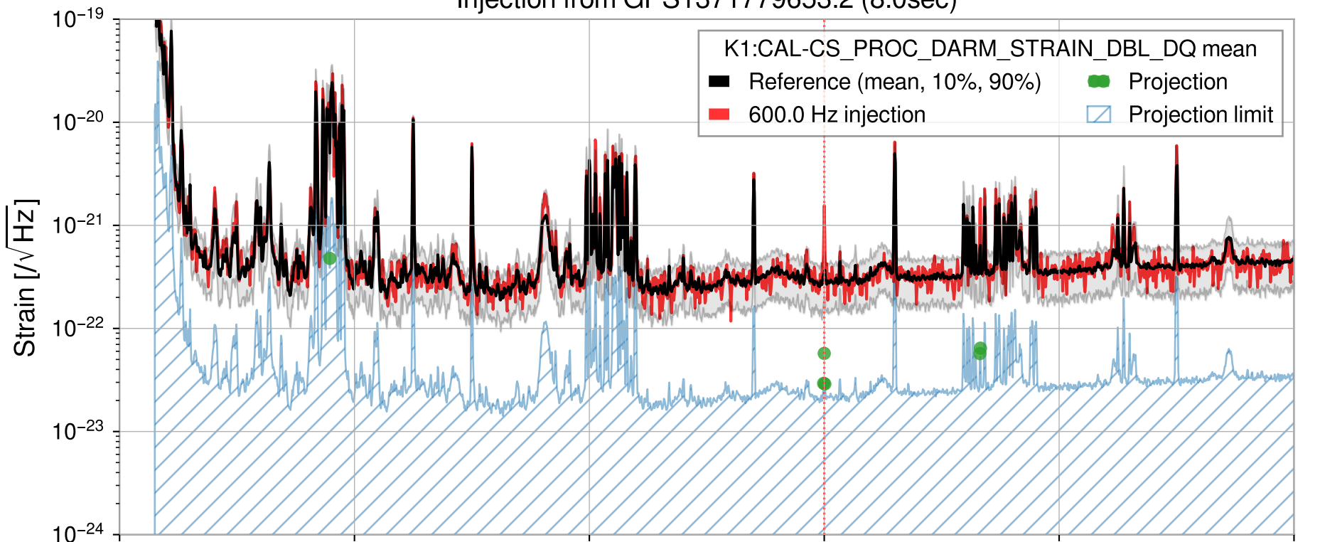
Injection from GPS1371779653.2 (8.0sec)
