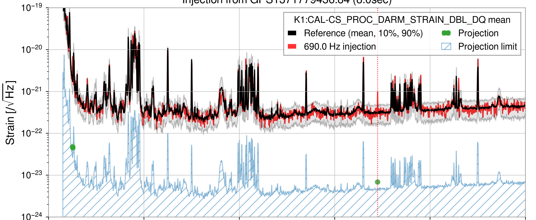
Injection from GPS1371779436.84 (8.0sec)
