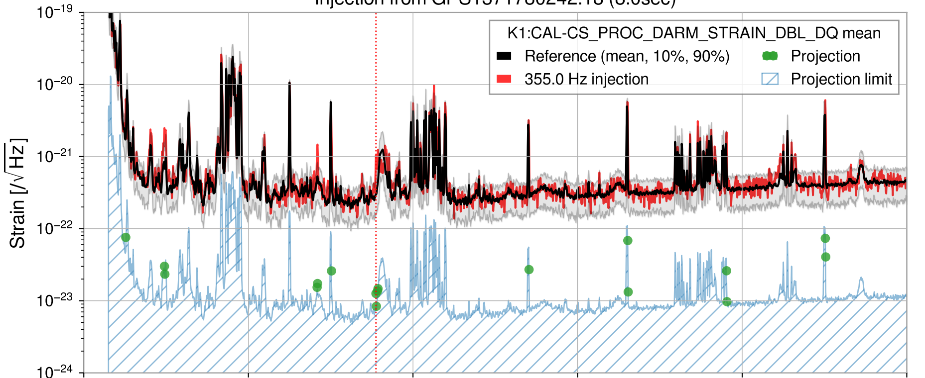
Injection from GPS1371780242.18 (8.0sec)
