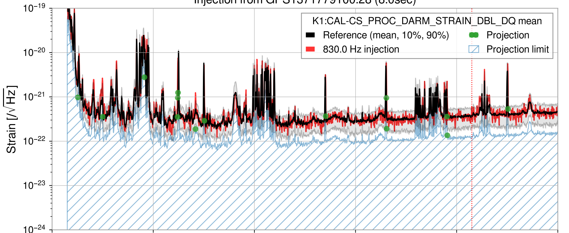
Injection from GPS1371779100.28 (8.0sec)
