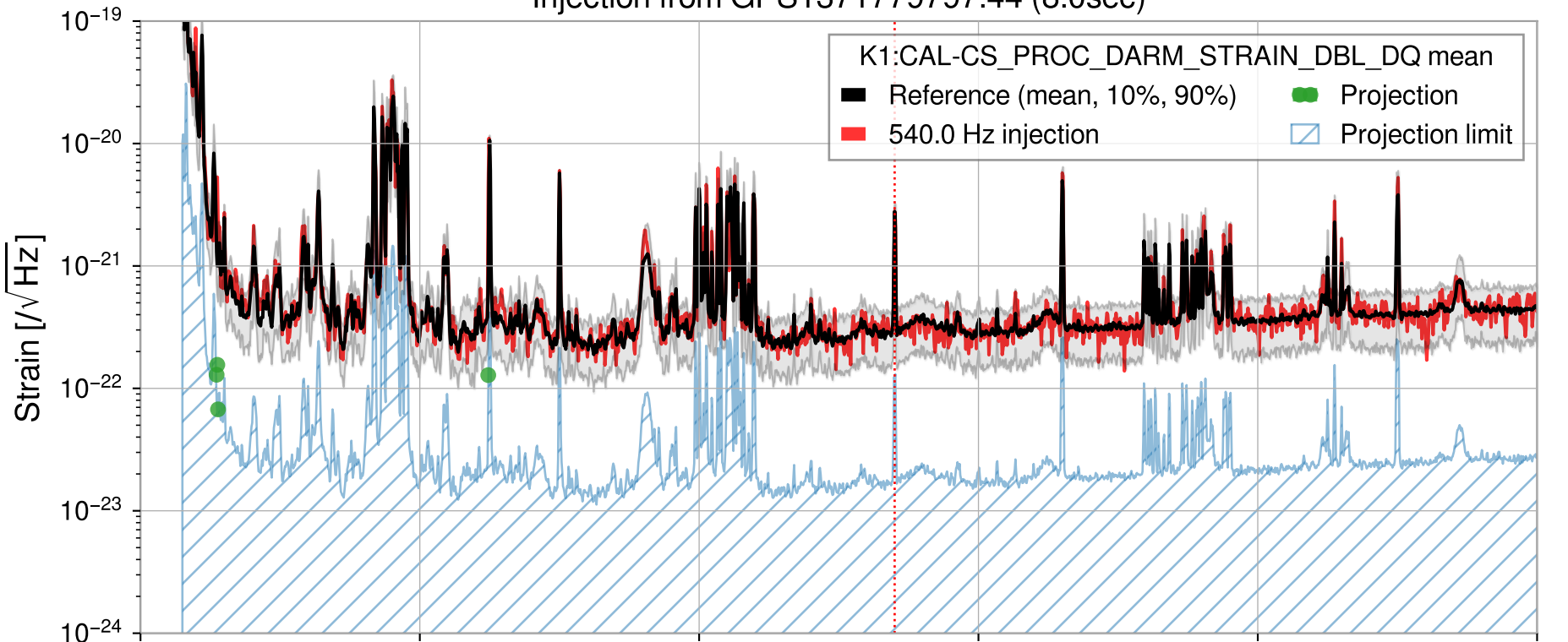
Injection from GPS1371779797.44 (8.0sec)
