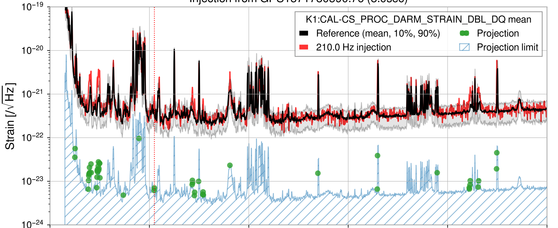
Injection from GPS1371780590.76 (8.0sec)
