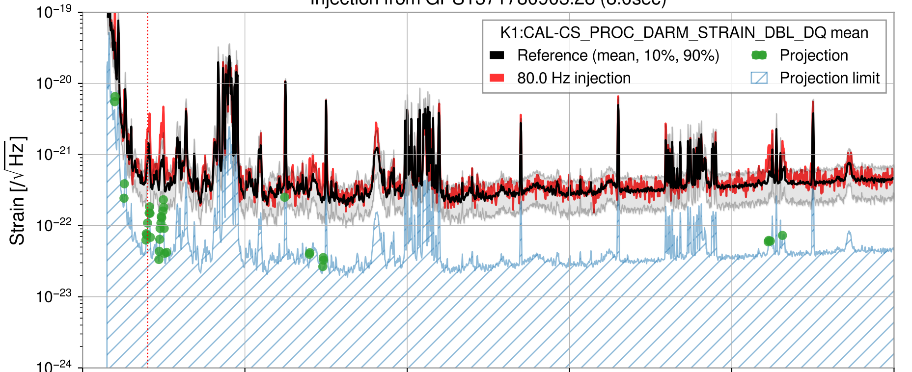
Injection from GPS1371780903.28 (8.0sec)
