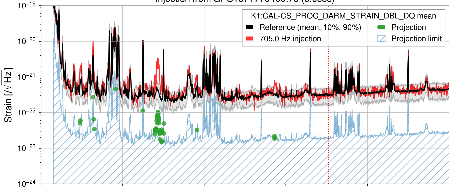
Injection from GPS1371779400.78 (8.0sec)
