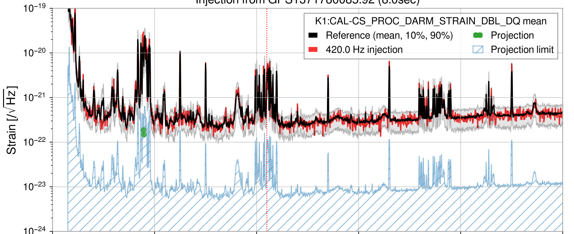
Injection from GPS1371780085.92 (8.0sec)
